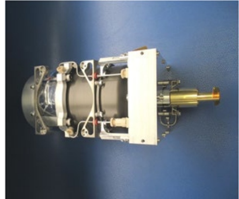
Figure 4.18: Comet-1000. Credit: Bradford Space.
