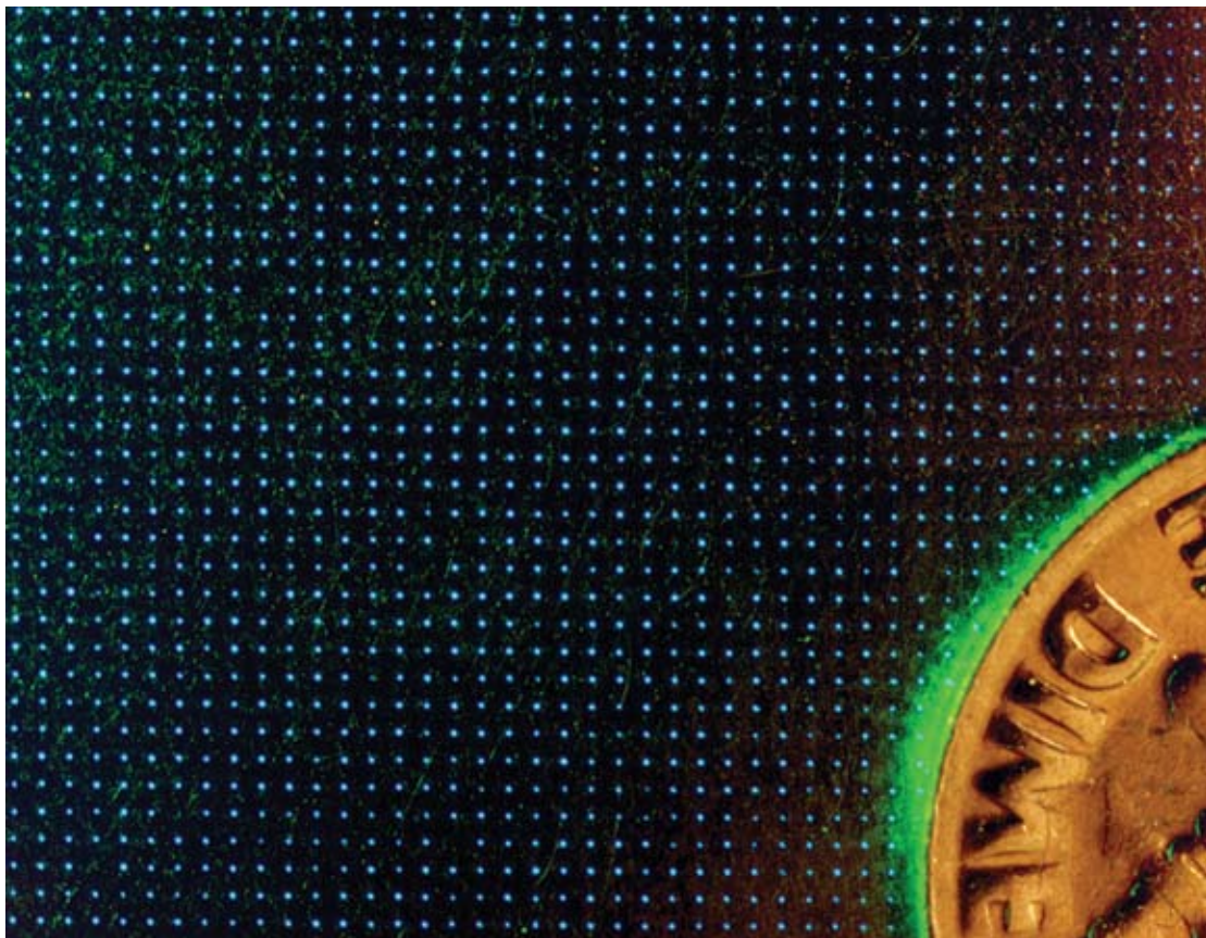
Size of holes in F-16XL test glove compared with a dime.
