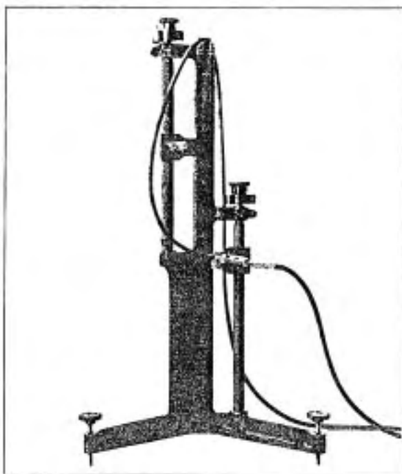
FIG. 8—THE MICRO MANOMETER
