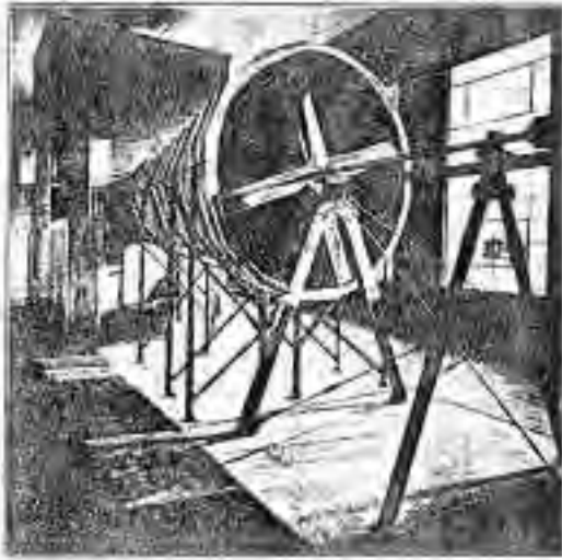
FIG. 3. THE LOWER STORY OF THE EXPERIMENTAL CHAMBER.
