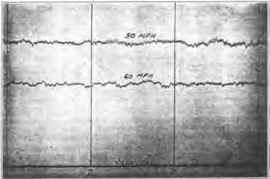
FIG. 20.—VELOCITY VARIATIONS IN LARGE TUNNEL, WITH DRIVING MOTOR CONNECTED TO A 25 H. W. GASOLINE GENERATING SET.
