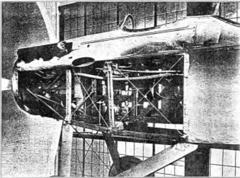
Fig. 11 ENGINE STARTER
