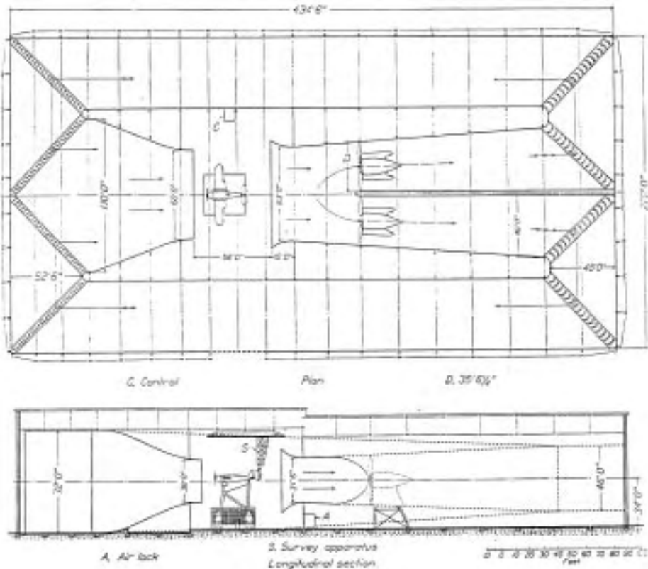
FIGURE 1.—Plan and elevation of the lock.
