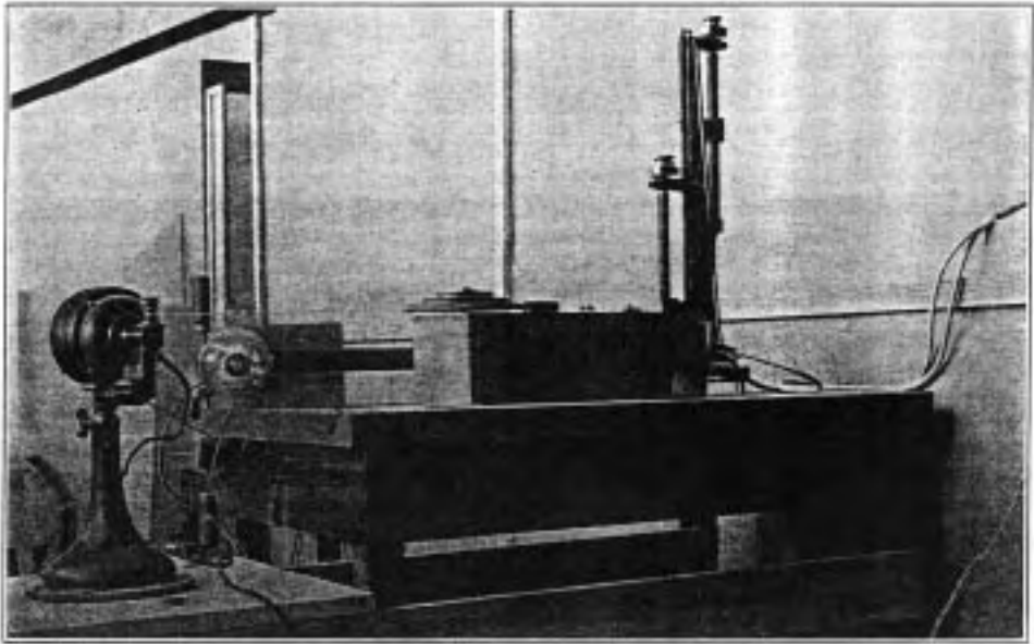
FIG. 3.—RECORDING AIR SPEED METER WITH ILLUMINATING AND RECORDING APPARATUS.
