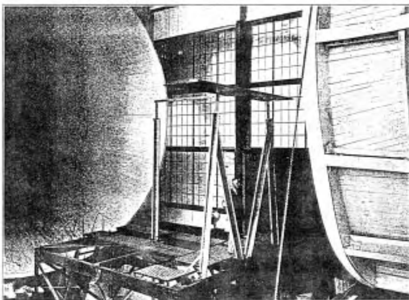
FIG. 18 ACCURACY
