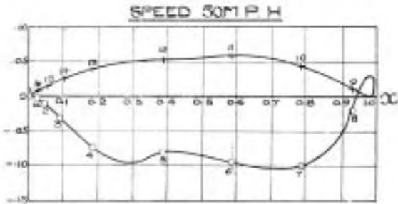
REPORT BY 287 MOMENT COEFFICIENT DIAGRAMS FIG. 9 ABSCISSAE ARE VALUES OF \alpha ORDINATES ARE PRODUCTS OF (PRESSURE/ \rho V^2 ) AND \alpha
