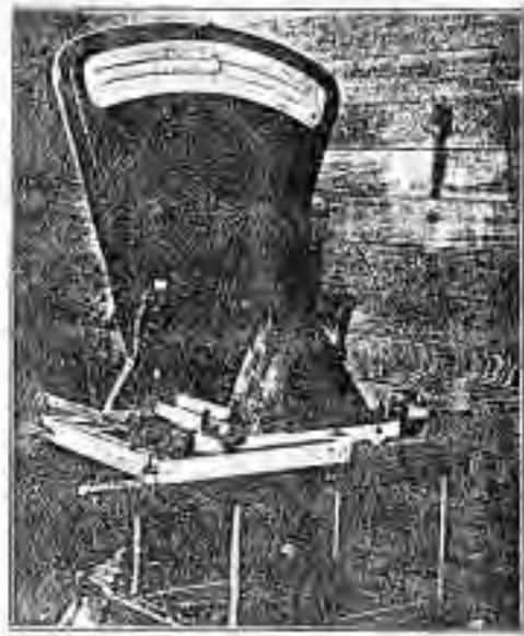
Fig. 7. Wing mounted on the center of pressure balance, showing the method of support by wires.
