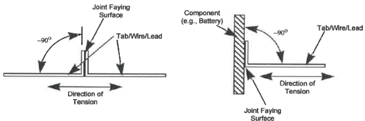
Figure 1 - Peel Test Examples
