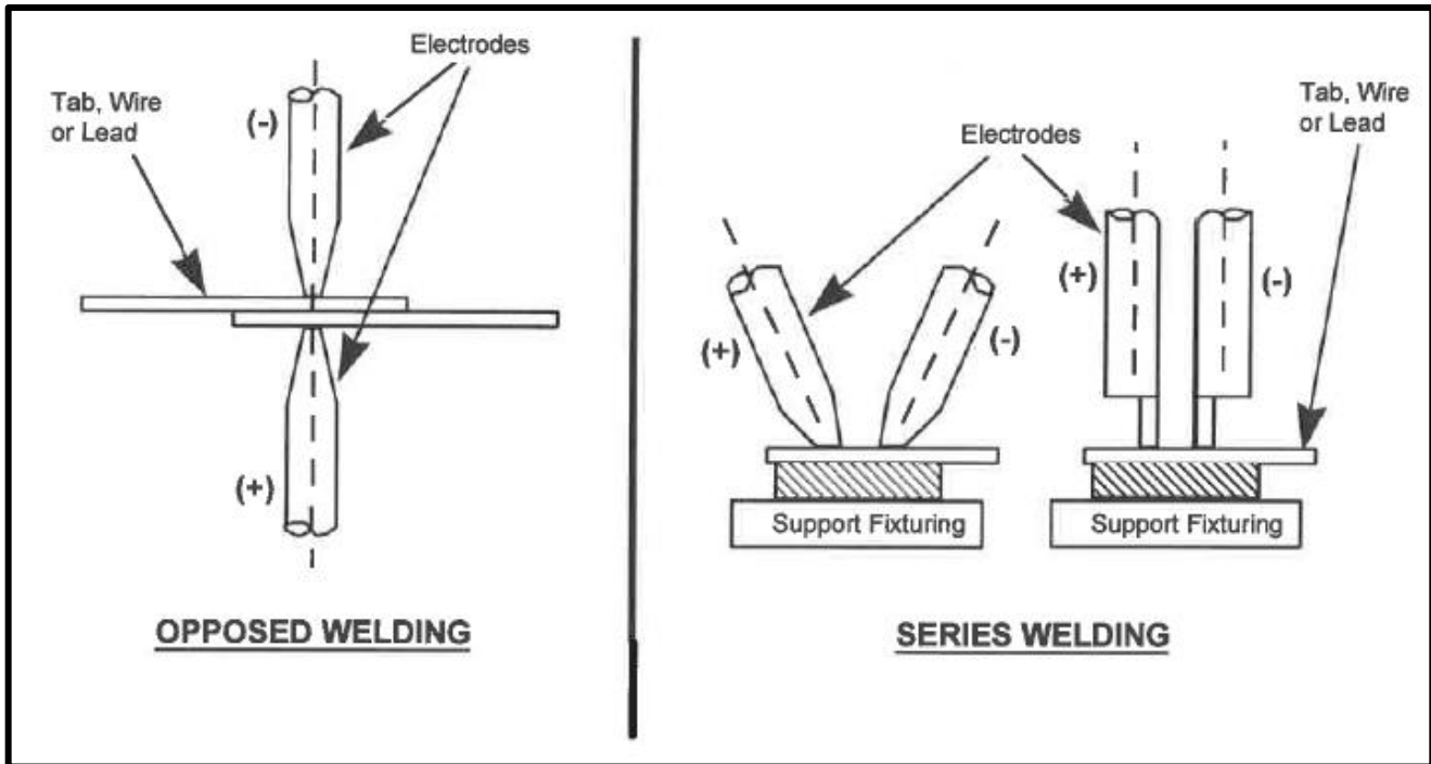
Figure 1: Opposed and Series Welding
