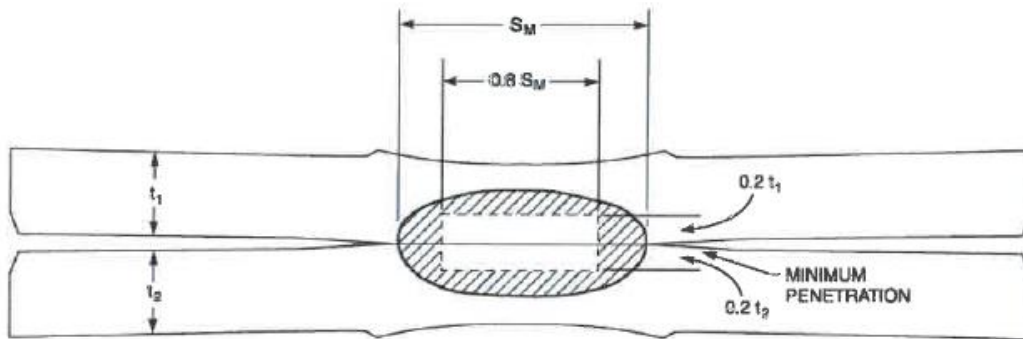
Figure 3: Metallographic Cross-Section after Etching
