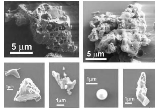
Source: Micro-Morphology and Toxicological Effects of Lunar Dust
