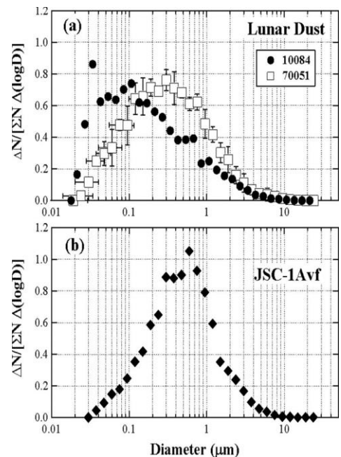
Source: Park et al, 2008 Characterization of Lunar Dust for Toxicological Studies: Particle Size Distribution
