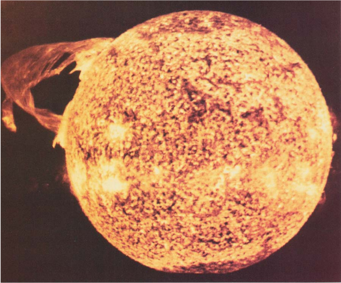
Photograph of a solar flare taken by the crew of the Skylab 4 mission.
