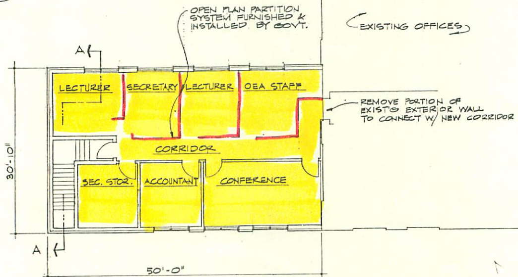
SECOND FLOOR PLAN SCALE 1/8" = 1'-0"
