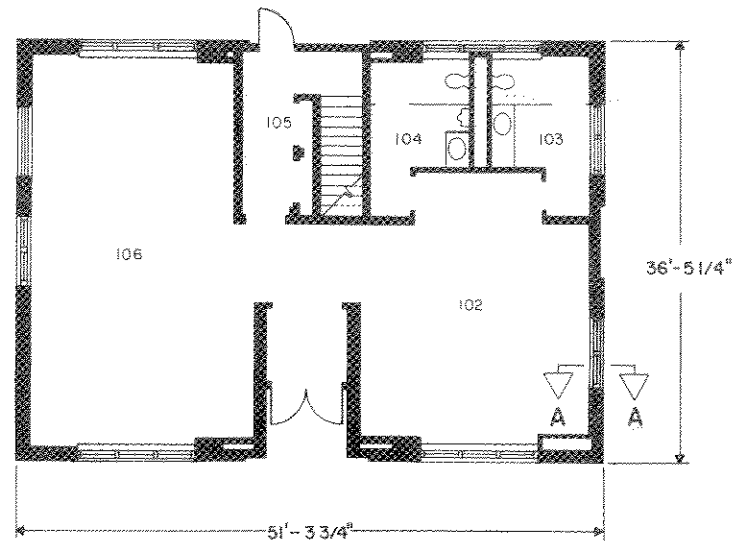
FIRST FLOOR PLAN 1,693 SQ. FT.
