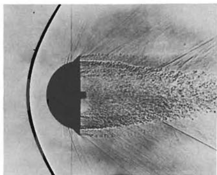
Blunt body concept, 1957
