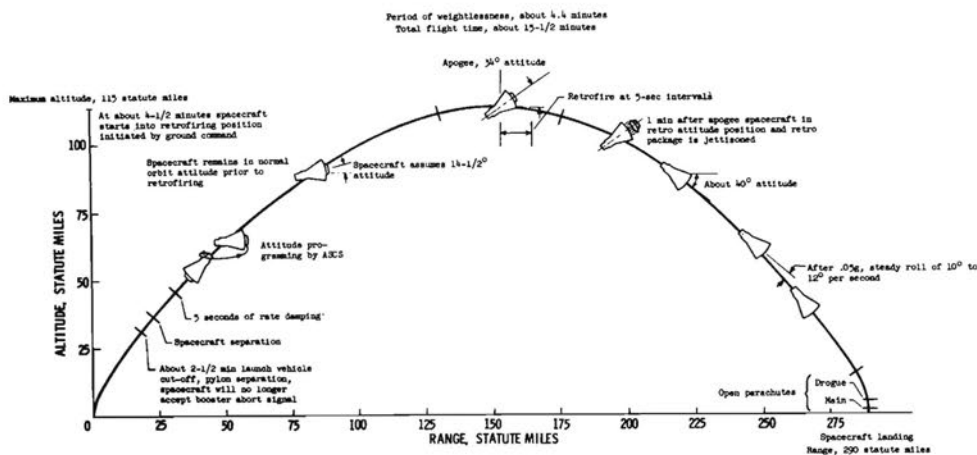
Normal sequence of events for Mercury-Redstone flight.
