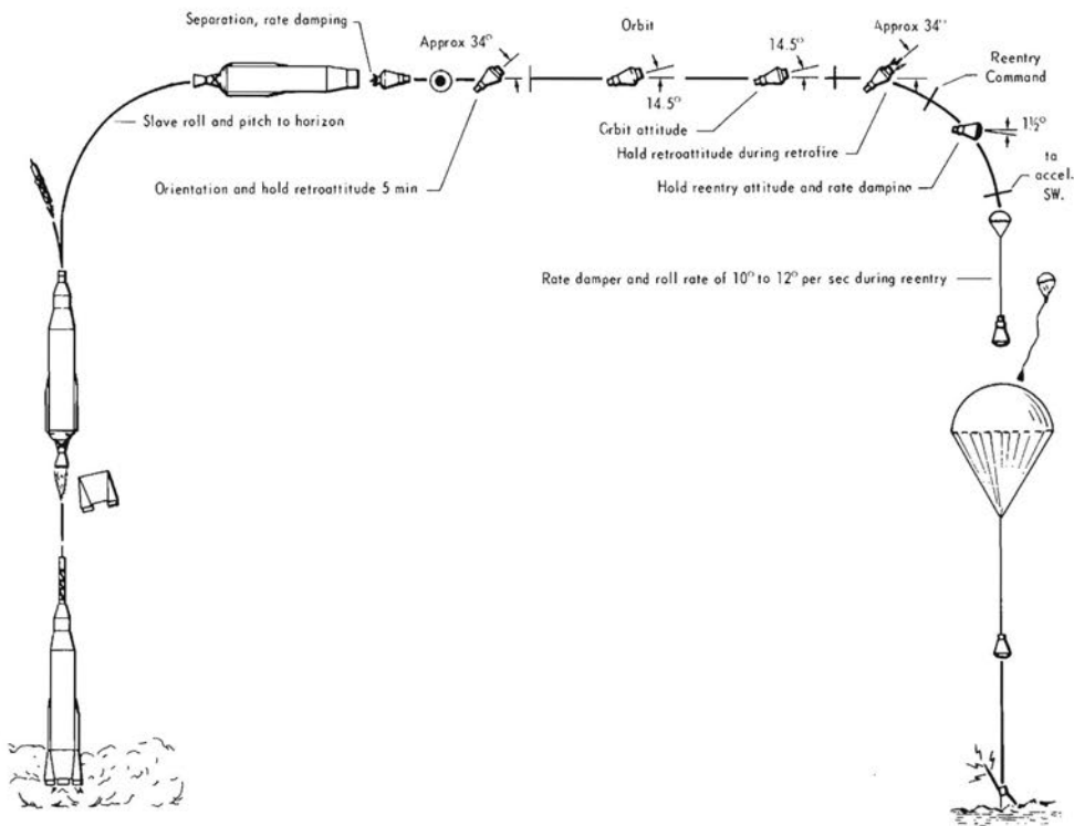
Project Mercury normal orbital mission profile.
