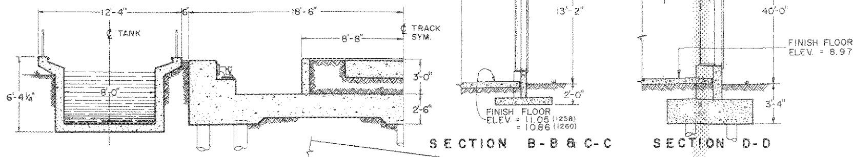
SECTION A - A PAVED TEST STRIP FACILITY NO. 1257-A
