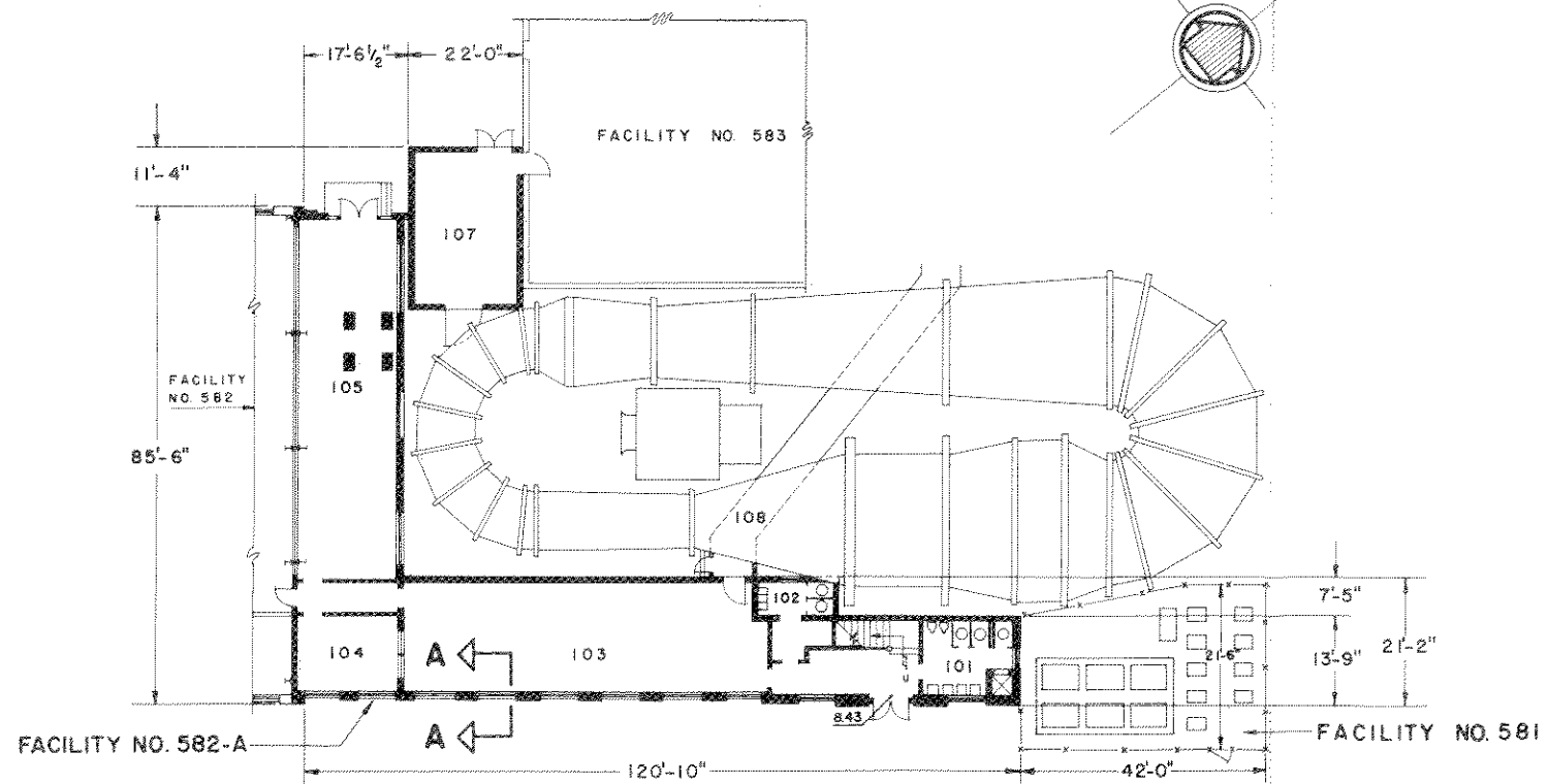
FIRST FLOOR PLAN 4,050 SQ. FT.
