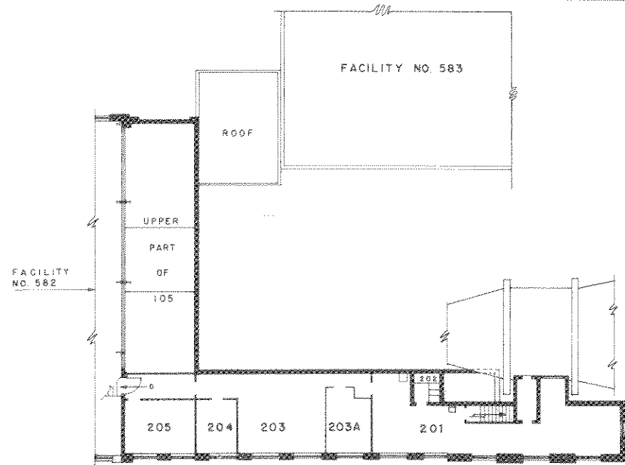
SECOND FLOOR PLAN 2297 SQ. FT.
