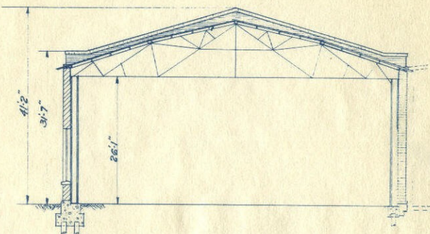
SECTION A-A SCALE \frac{1}{8} = 1'-0"
