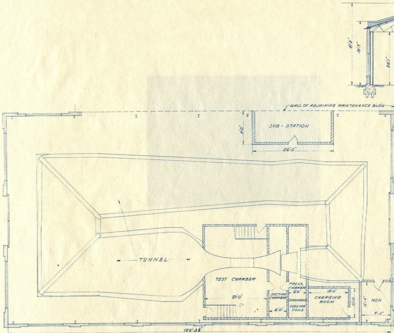
FLOOR PLAN SCALE \frac{3}{16} = 1'-0"
