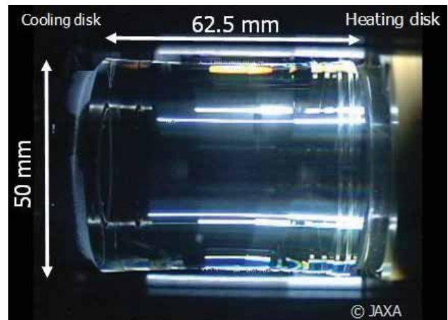
Large liquid bridge of silicone oil (JAXA image).
