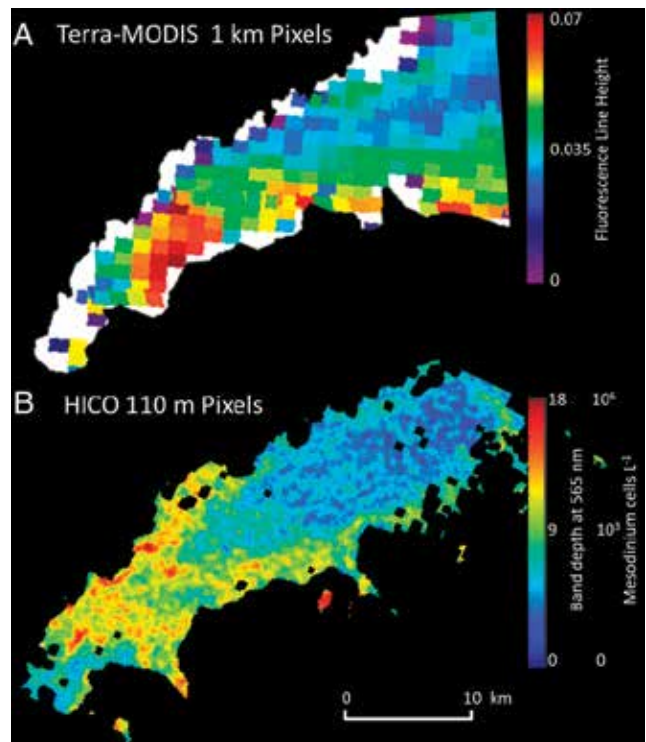
(A) Image of WLIS at a resolution of 1 km from the MODIS Terra sensor shows an elevated Chl a fluorescence patch on September 23, 2012, but the type of bloom cannot be distinguished from the limited spectral bands. (B) In contrast, hyperspectral HICO imagery from the International Space Station reveals characteristic yellow fluorescence due to phycoerythrin pigment within the enslaved chloroplasts of the ciliate M. rubrum . Dense and patchy near-surface blooms of this motile and actively photosynthesizing mixotrophic marine protist ( >1 \times 10^6 cells per liter) periodically dominate primary productivity in the region.
