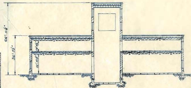
SECTION B-B SCALE 1/16" = 1'-0"
