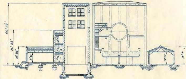
SECTION A-A SCALE 1/16" = 1'-0"
