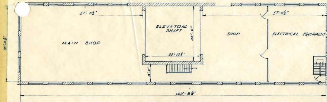
SECOND FLOOR PLAN SCALE 1/8" = 1'-0"
