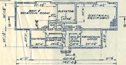
FIRST FLOOR PLAN SCALE 1" = 20'-0"
