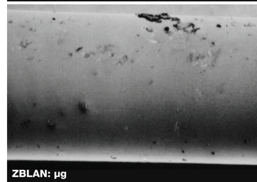
Two collaborative projects will investigate the advantages of manufacturing ZBLAN-based optical fiber in microgravity. These scanning electron microscope images show the surface of ZBLAN fibers pulled in microgravity ( \mu g) and on Earth (1g). Manufacturing in microgravity may help sidestep the crystallization that occurs in Earth-based processing. Credits: NASA
