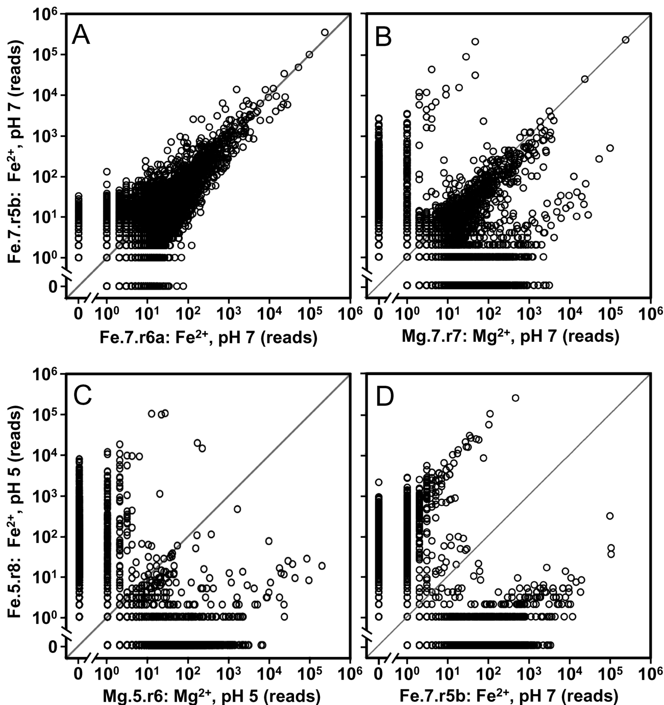
Figure 2. Impact of ion identify and pH on sequence abundance. Each point on the scatter plots represents the abundance of a unique sequence in two different populations. For plots (A) and (B) the y-axis is the sequence abundance within a random sample of 10^6 reads from a population evolved in the presence of \text{Fe}^{2+} at pH 7 (Fe.7.r5b) plotted against the sequence abundance in populations (A) evolved under the same conditions along an independent trajectory (Fe.7.r6a), and (B) evolved in the presence of \text{Mg}^{2+} at pH 7 (Mg.7.r7). For plots (C) and (D) the y-axis is the sequence abundance within a population evolved in the presence of \text{Fe}^{2+} at pH 5 (Fe.5.r8) plotted against the abundance of sequences in populations (C) evolved in the presence of \text{Mg}^{2+} at pH 5 (Mg.5.r6) and (D) evolved in the presence of \text{Fe}^{2+} at pH 7 (Fe.7.r5b).
