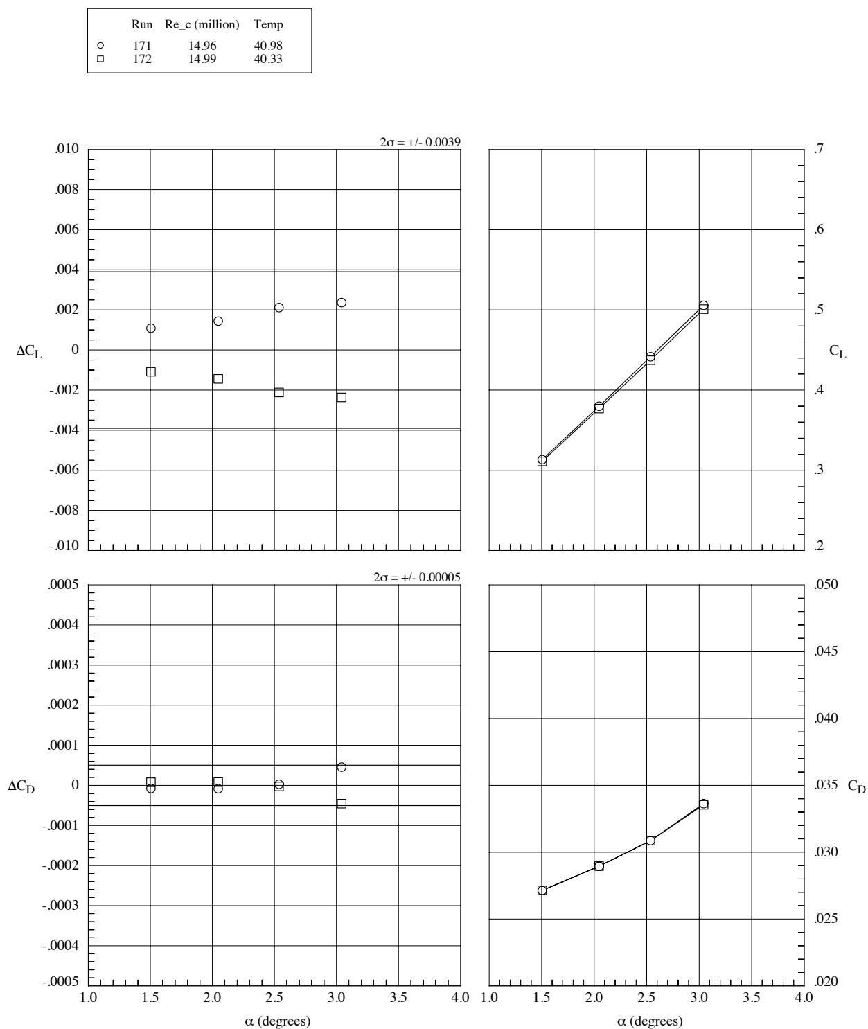
Fig. 14. Data repeatability, M_\infty = 0.86 , Re_c = 15 million, T_t = 40^\circ\text{F} , q_\infty = 1775 psf. Solid line indicates 2-sigma limits based on the residual data.
