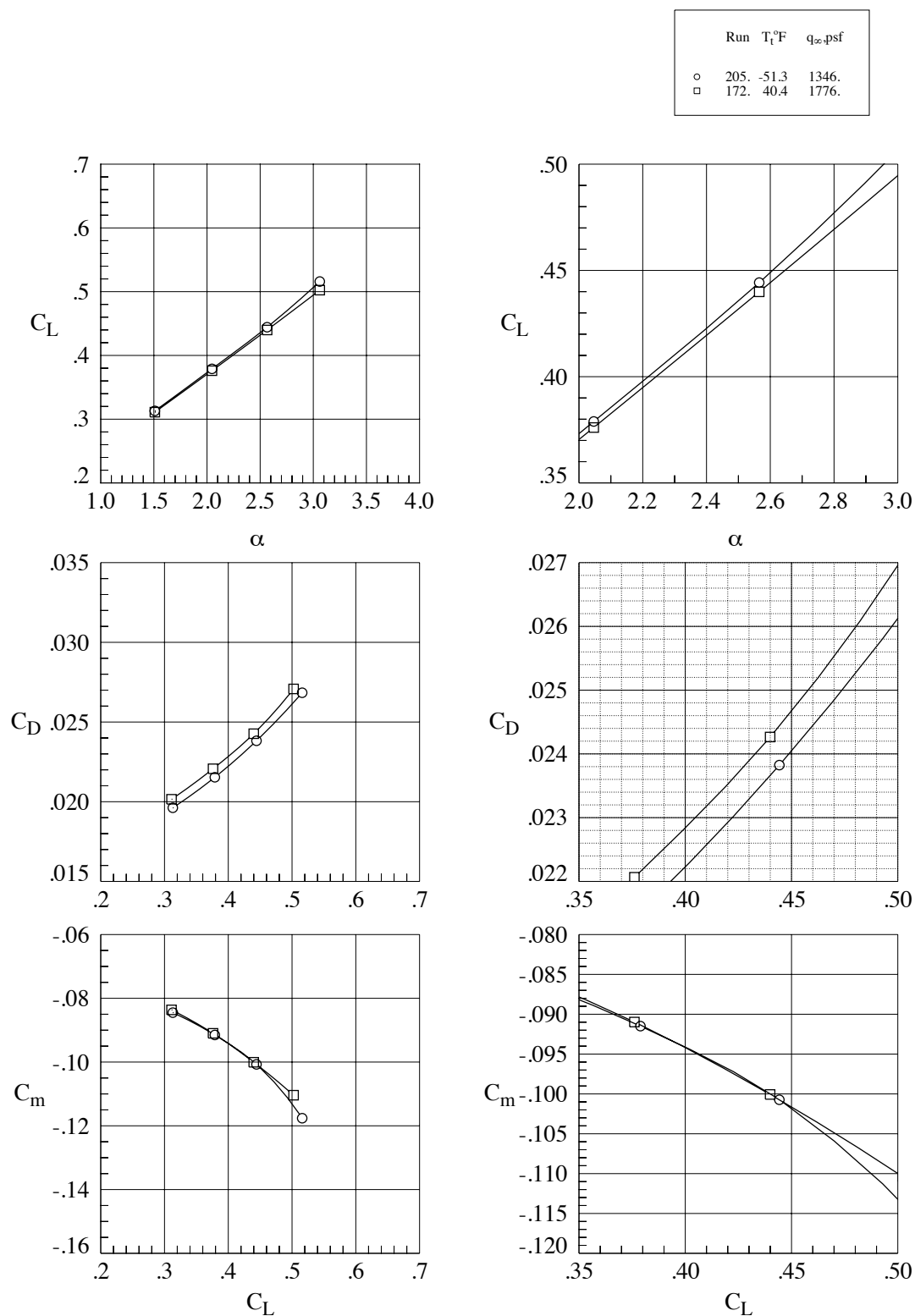
Fig. 24. Aeroelastic effects, M_\infty = 0.86 , Re_c = 15 million.
