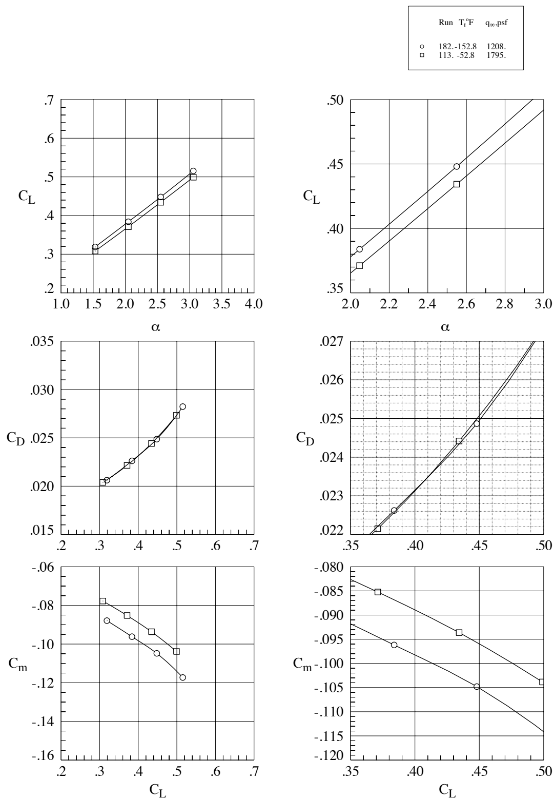
Fig. 25. Aeroelastic effects, M_{\infty} = 0.86 , Re_c = 20 million.
