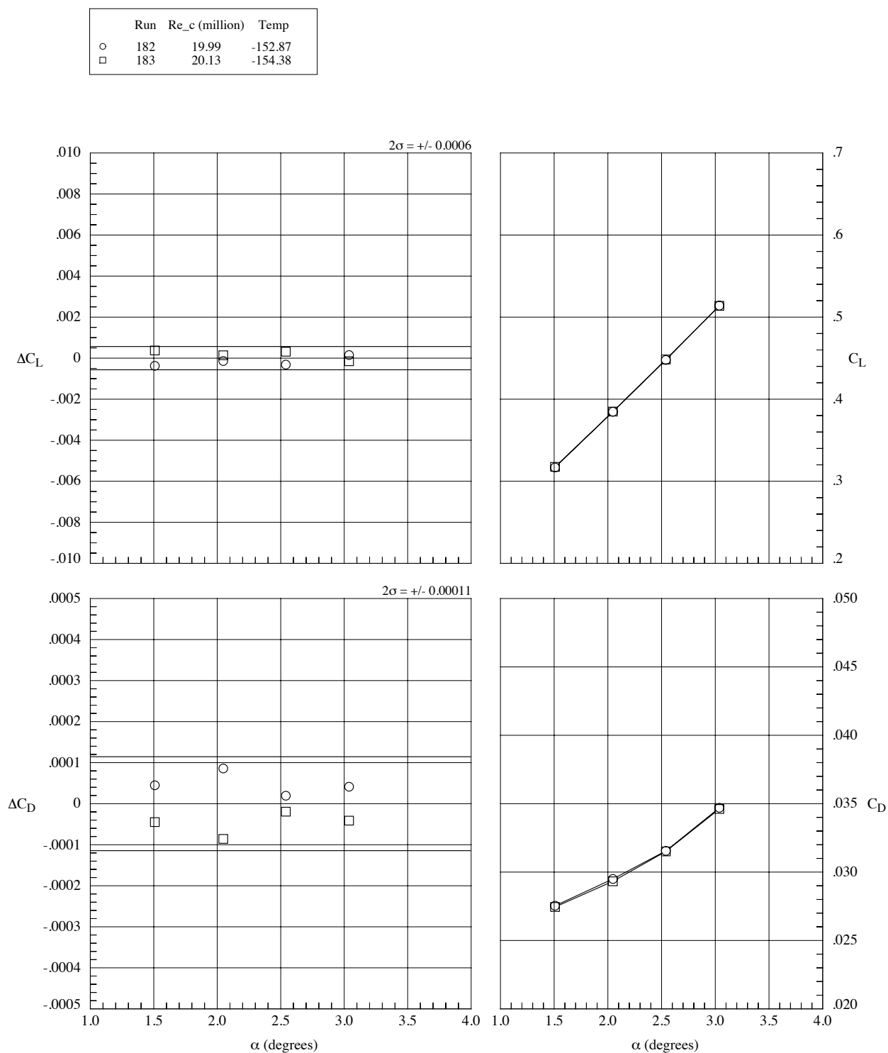
Fig. 18. Data repeatability, M_\infty = 0.86 , Re_c = 20 million, T_t = -153^\circ\text{F} , q_\infty = 1208 psf. Solid line indicates 2-sigma limits based on the residual data.
