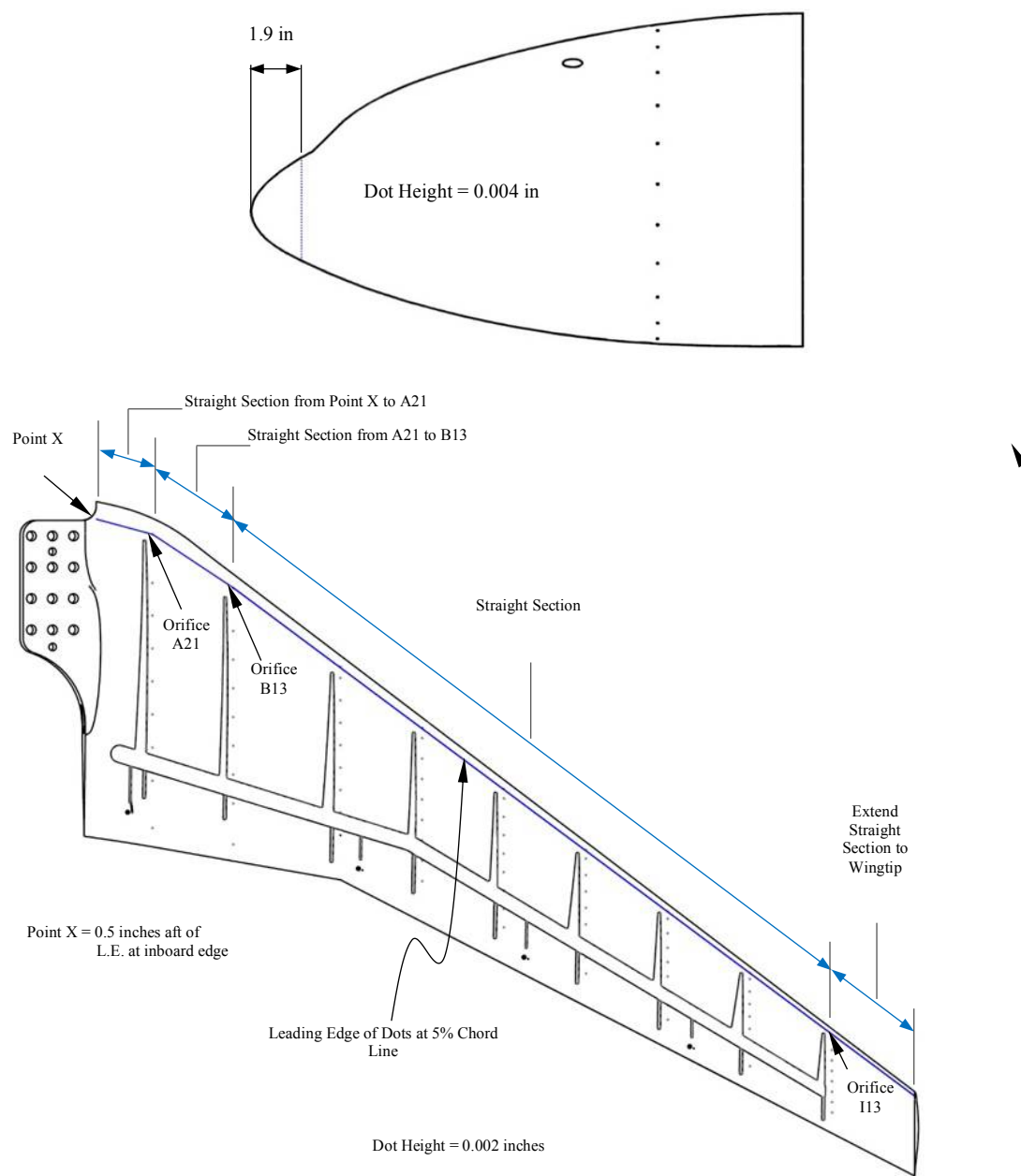
Fig. 10. Location of trip dots on the fuselage nose and the lower surface of the CRM-NLF semispan wing.
