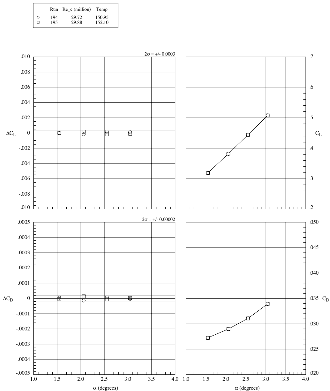
Fig. 19. Data repeatability, M_\infty = 0.86 , Re_c = 30 million, T_t = -153^\circ\text{F} , q_\infty = 1814 psf. Solid line indicates 2-sigma limits based on the residual data.
