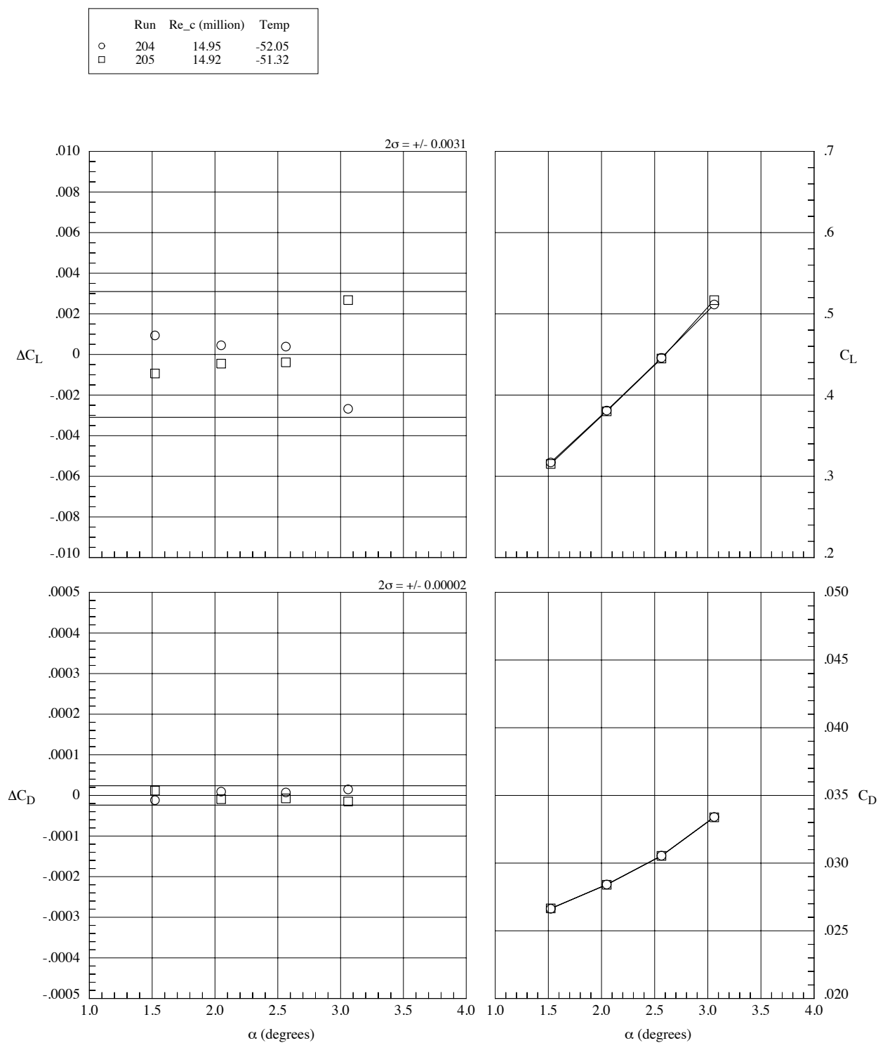
Fig. 15. Data repeatability, M_\infty = 0.86 , Re_c = 15 million, T_t = -53^\circ\text{F} , q_\infty = 1346 psf. Solid line indicates 2-sigma limits based on the residual data.
