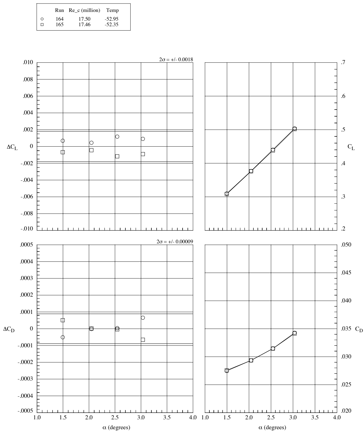
Fig. 16. Data repeatability, M_\infty = 0.85 , Re_c = 17.5 million, T_t = -53^\circ\text{F} , q_\infty = 1570 psf. Solid line indicates 2-sigma limits based on the residual data.
