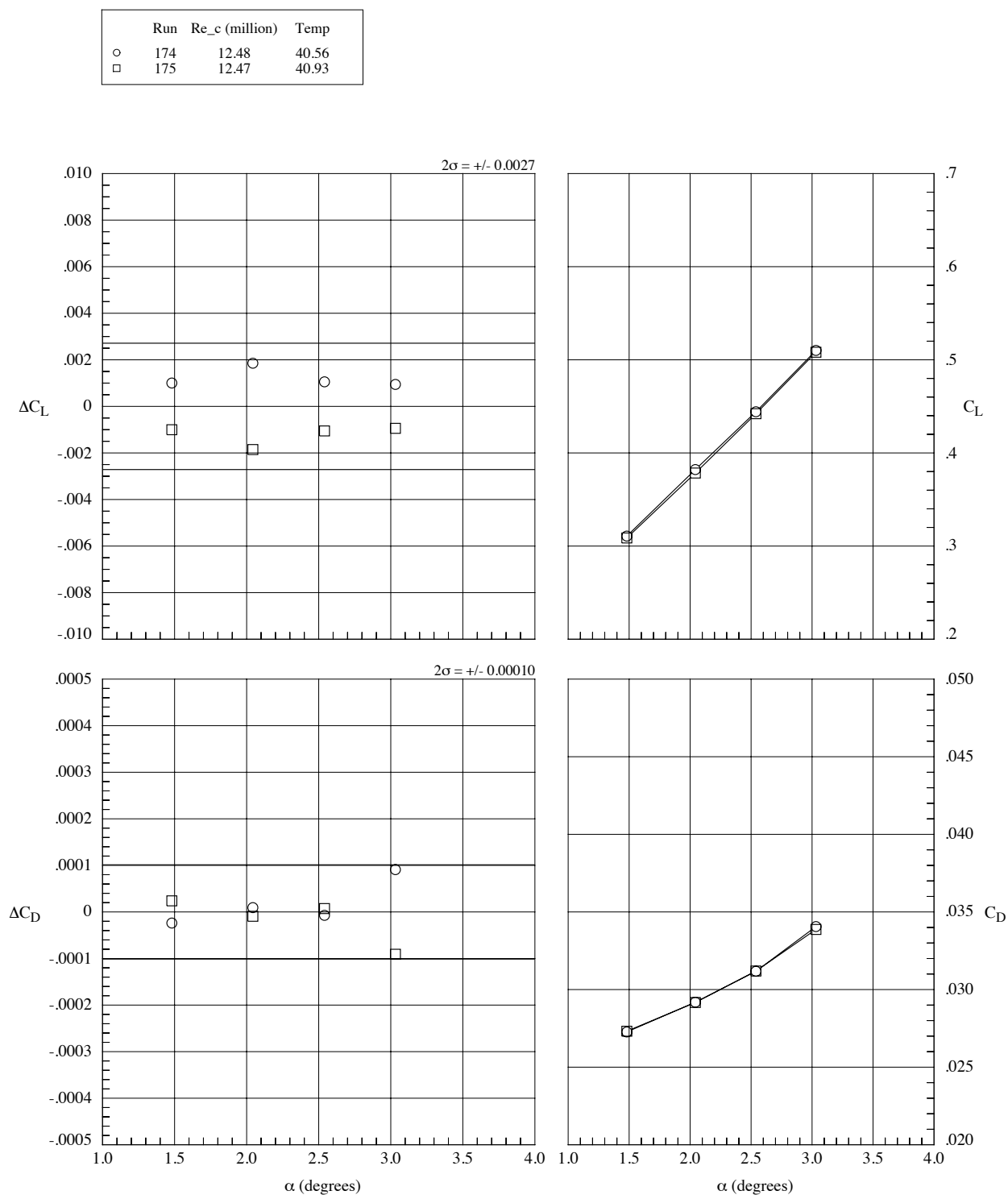
Fig. 12. Data repeatability, M_\infty = 0.86 , Re_c = 12.5 million, T_t = 40^\circ\text{F} , q_\infty = 1479 psf. Solid line indicates 2-sigma limits based on the residual data.
