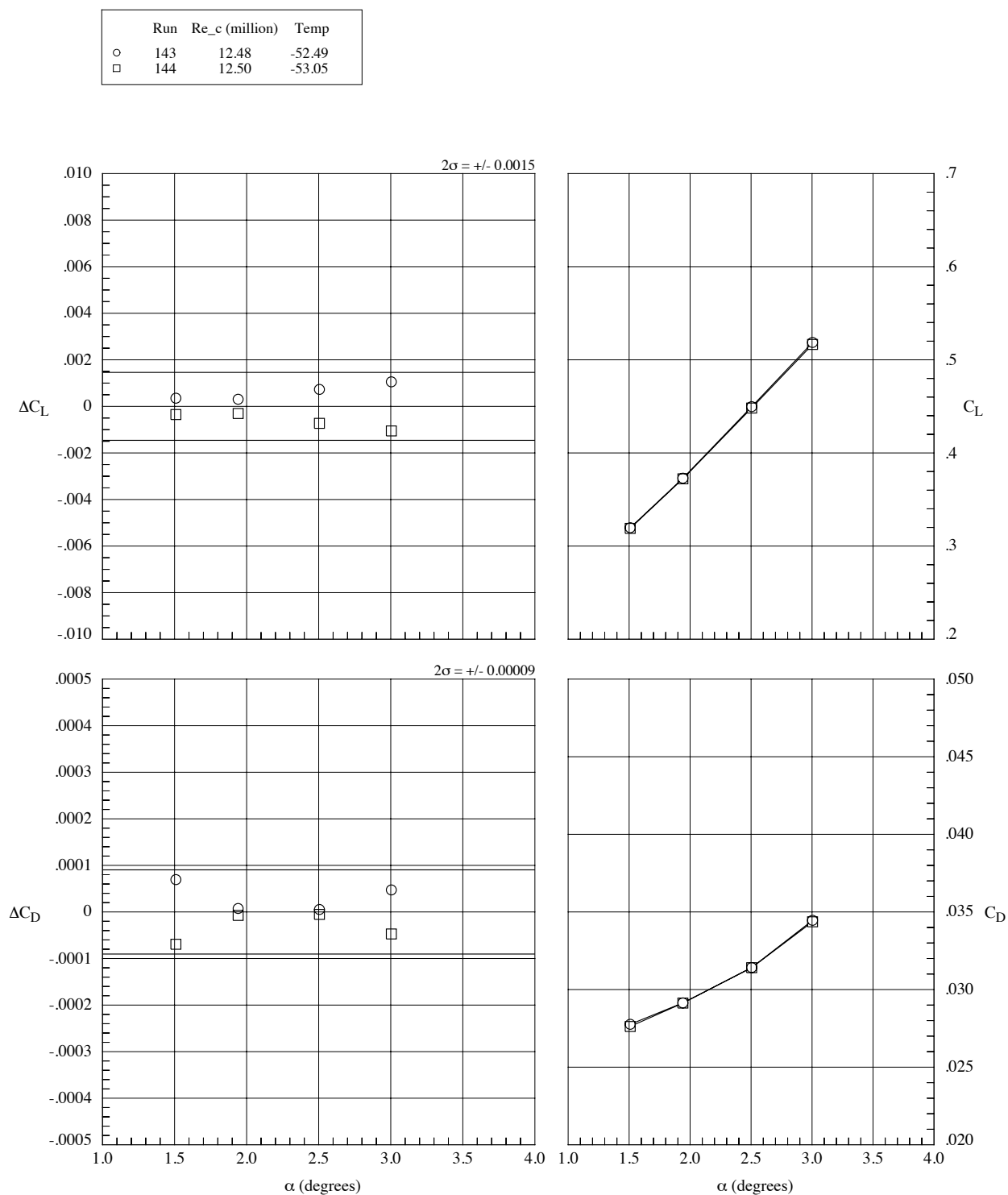
Fig. 13. Data repeatability, M_\infty = 0.86 , Re_c = 12.5 million, T_t = -53^\circ\text{F} , q_\infty = 1120 psf. Solid line indicates 2-sigma limits based on the residual data.
