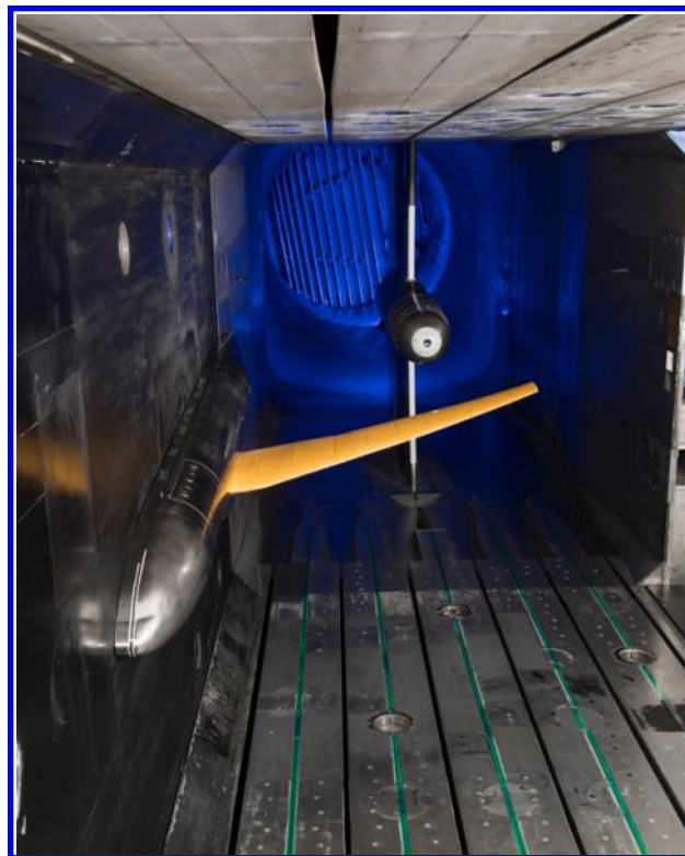
Fig. 7. Photo of the Common Research Model with Natural Laminar Flow wing in the National Transonic Facility.
