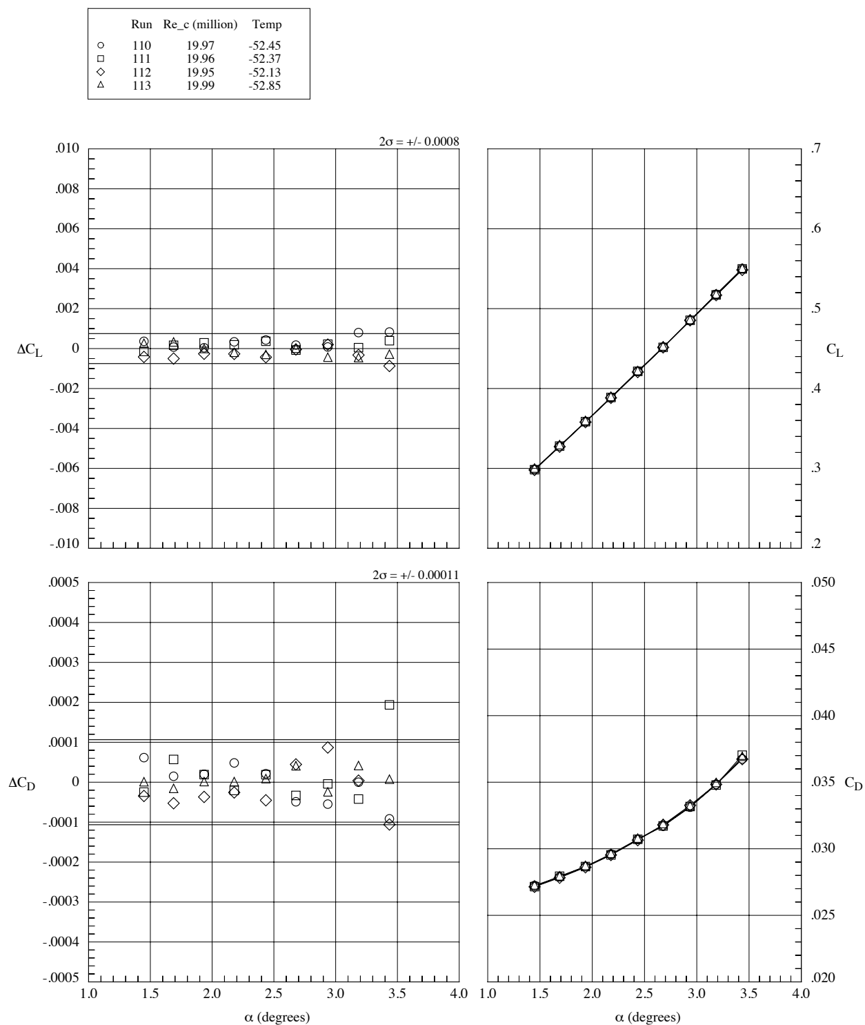
Fig. 17. Data repeatability, M_\infty = 0.86 , Re_c = 20 million, T_t = -53^\circ\text{F} , q_\infty = 1795 psf. Solid line indicates 2-sigma limits based on the residual data.
