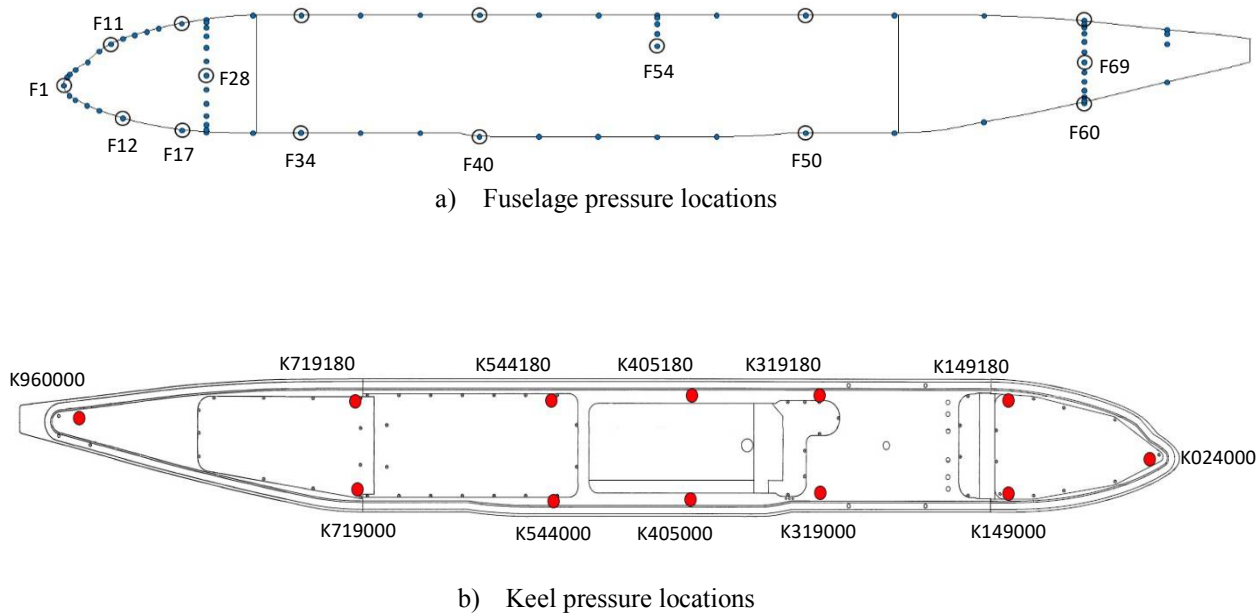
Fig. 9. Location of fuselage and keel pressures on the CRM-NLF semispan model.
