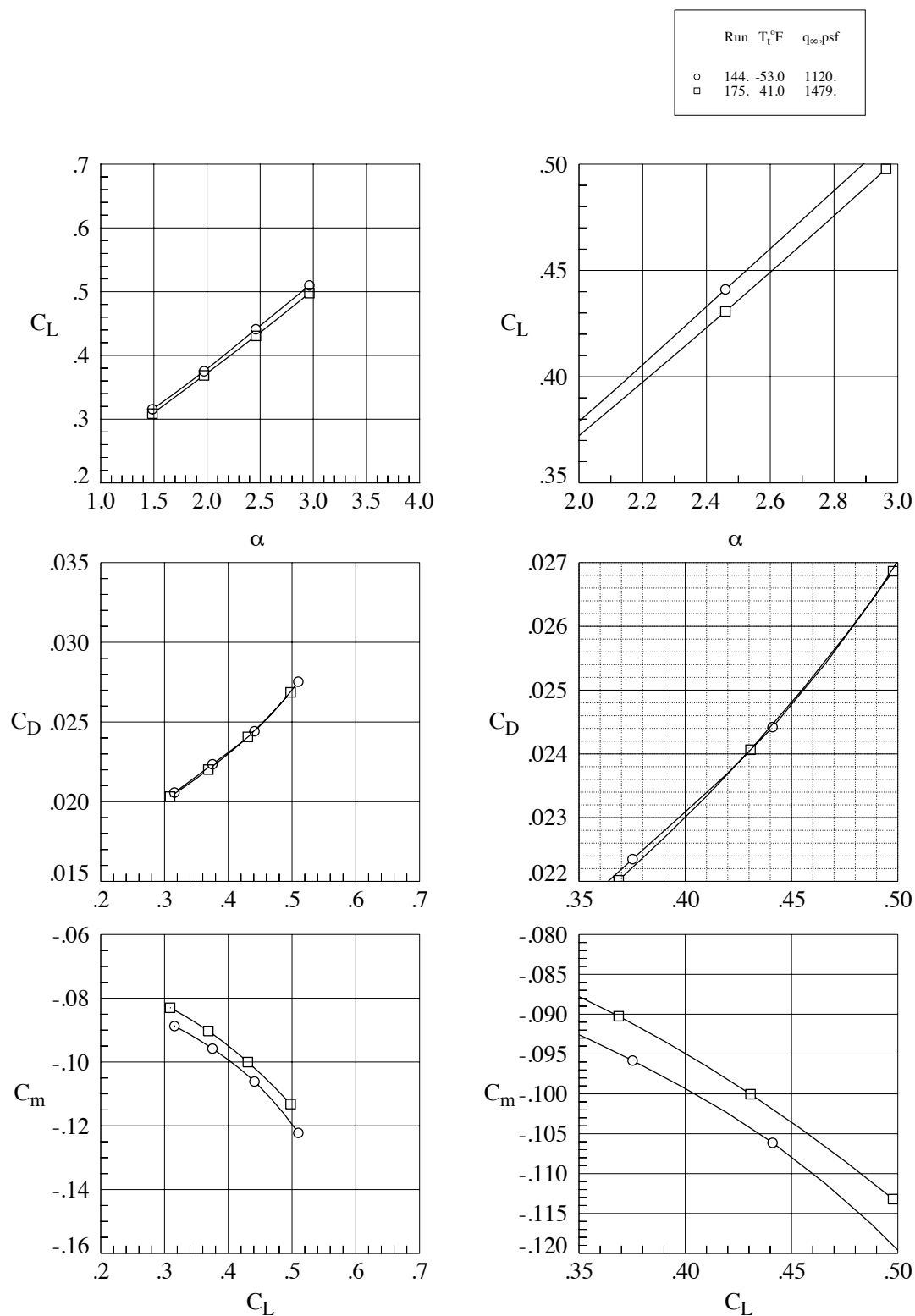
Fig. 23. Aeroelastic effects, M_{\infty} = 0.86 , Re_c = 12.5 million.
