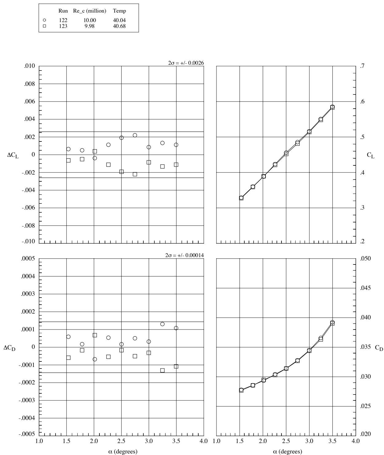
Fig. 11. Data repeatability, M_\infty = 0.86 , Re_c = 10 million, T_t = 40^\circ\text{F} , q_\infty = 1183 psf. Solid line indicates 2-sigma limits based on the residual data.
