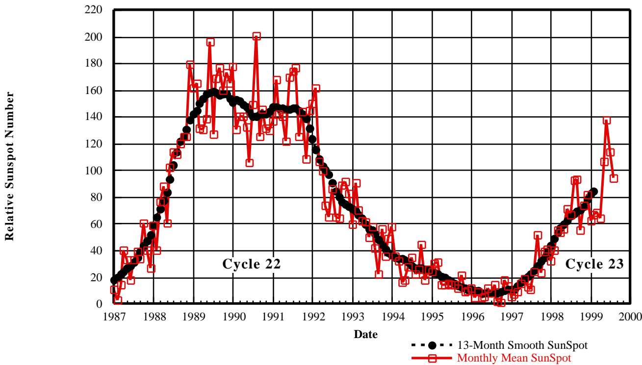
Figure 3. Plot of Recent Monthly Mean and 13-Month Smoothed Relative Sunspot Number
