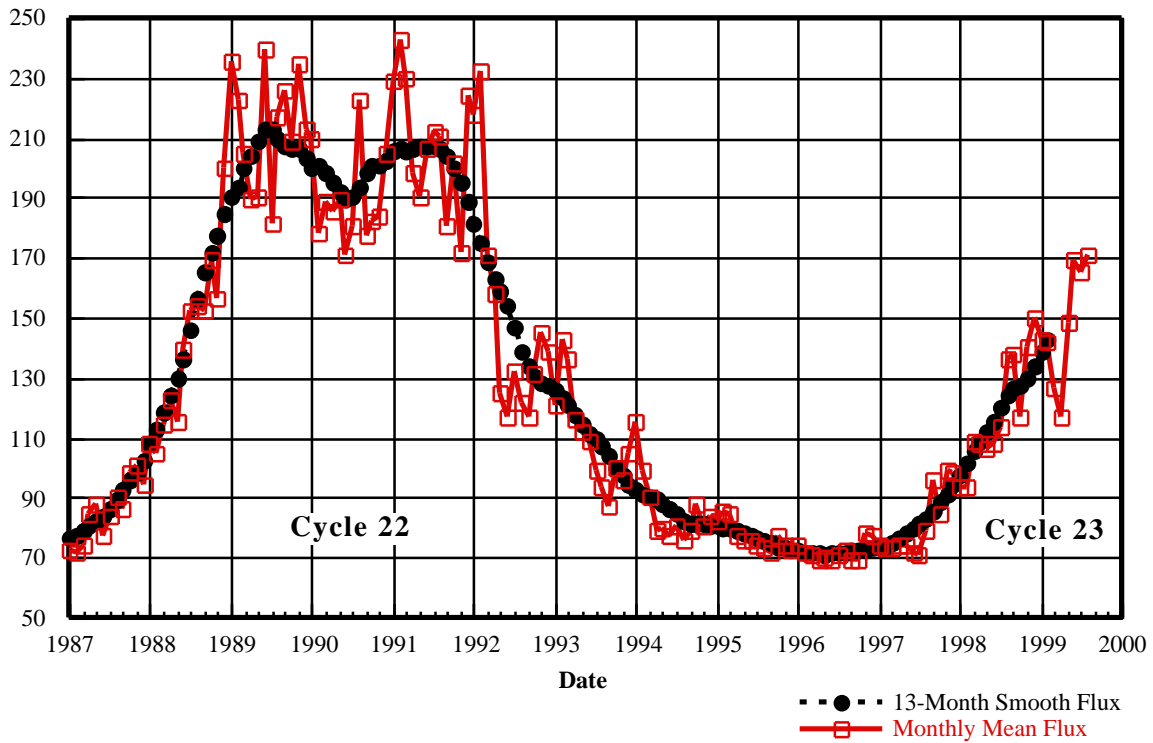
Figure 1. Plot of Recent Monthly Mean and 13-Month Smoothed Solar Flux
