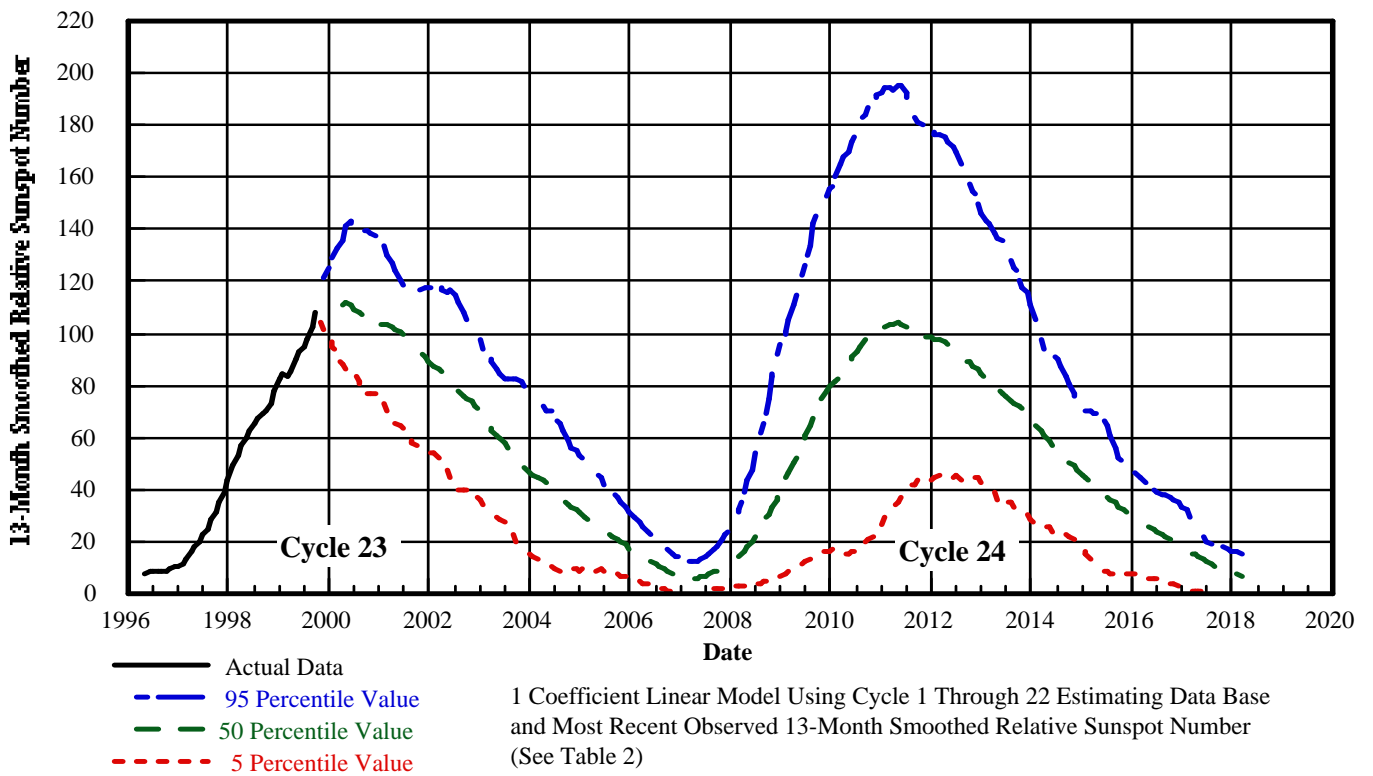
Figure 4. Estimate of 13-Month Smoothed Sunspot Number For Cycle 23* and Cycle 24
