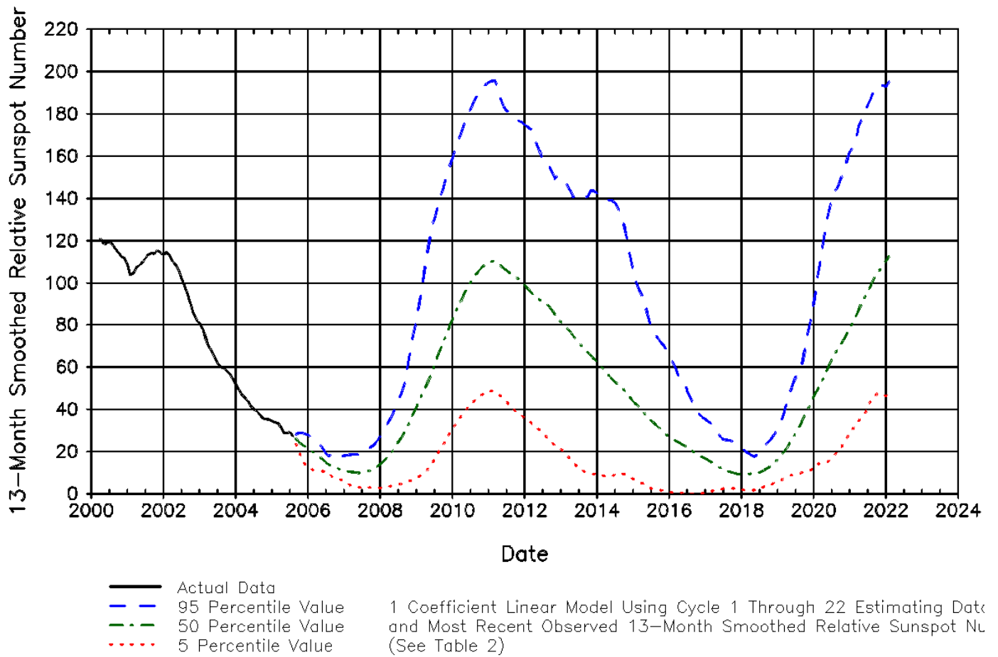
Figure 4. Estimate of 13-Month Smoothed Sunspot Number For Cycle 23* and Cycle 24
