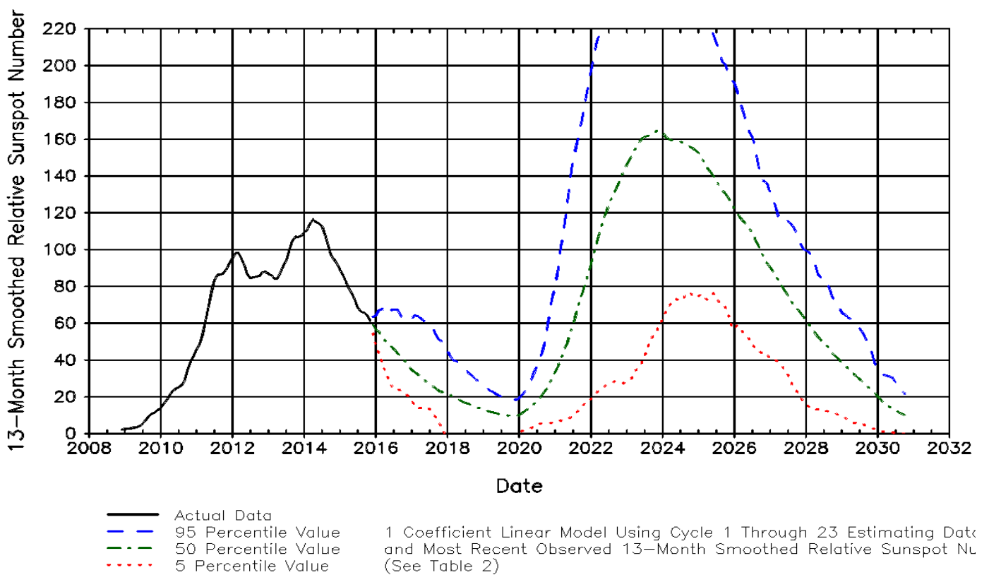
Figure 4. Estimate of 13-Month Smoothed Sunspot Number For Cycle 24* and Cycle 25
