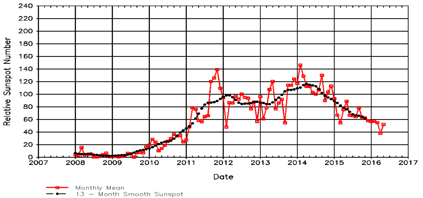
Figure 3. Plot of Recent Monthly Mean and 13-Month Smoothed Relative Sunspot Number
