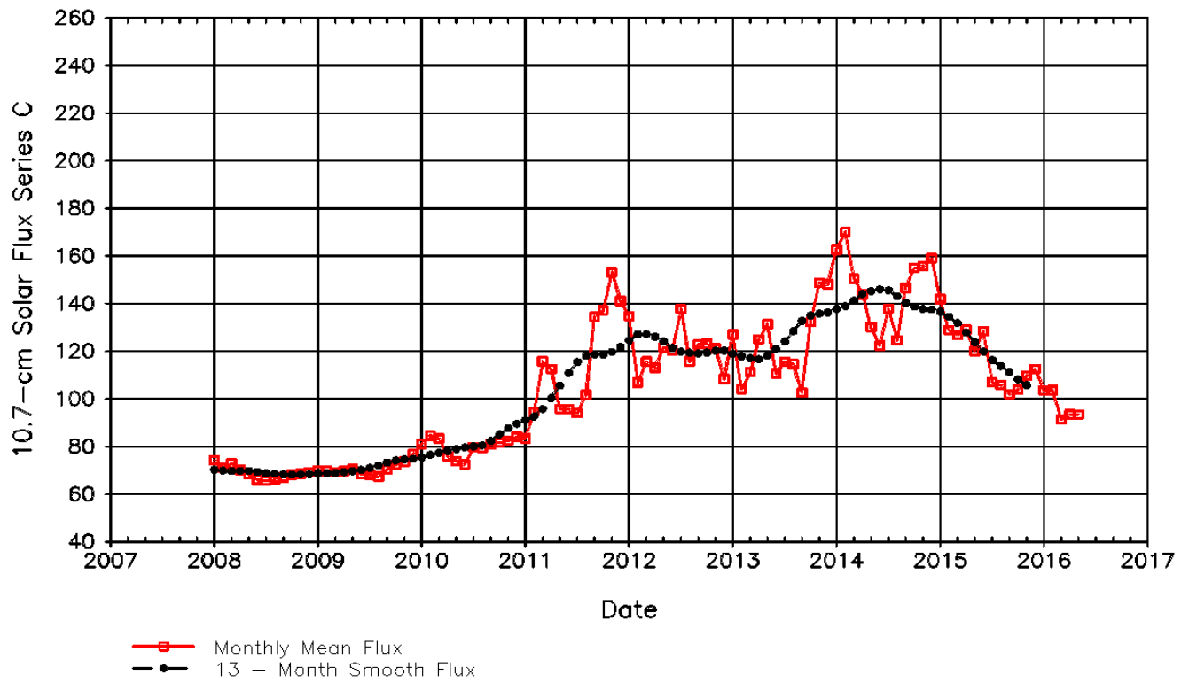
Figure 1. Plot of Recent Monthly Mean and 13-Month Smoothed Solar Flux
