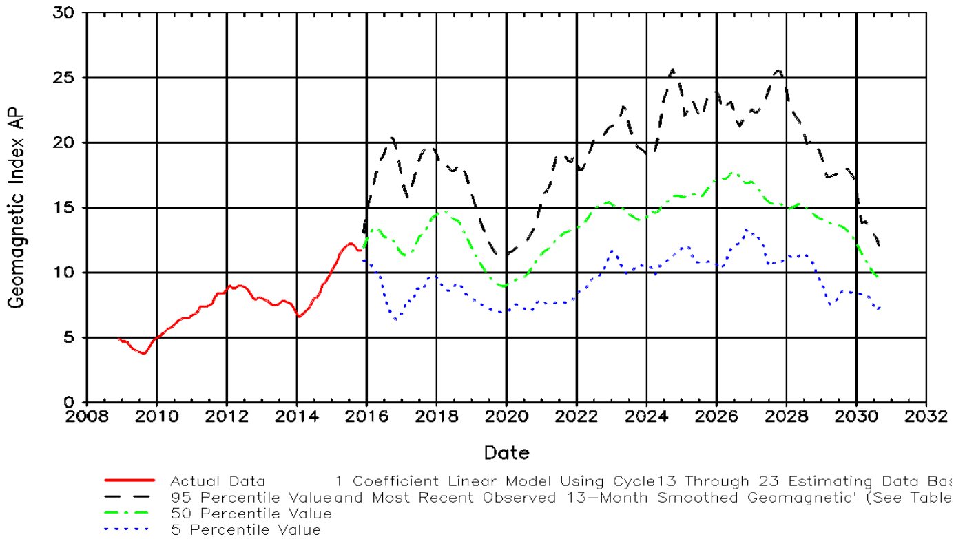
Figure 5. Estimate of 13-Month Smoothed Ap For Cycle 24* and Cycle 25
