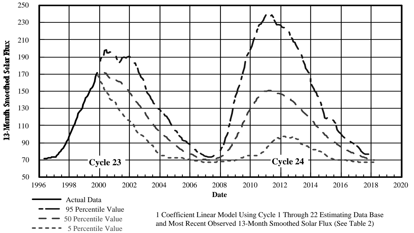
Figure 2. Estimate of 13-Month Smoothed Solar Flux For Cycle 23* and Cycle 24
