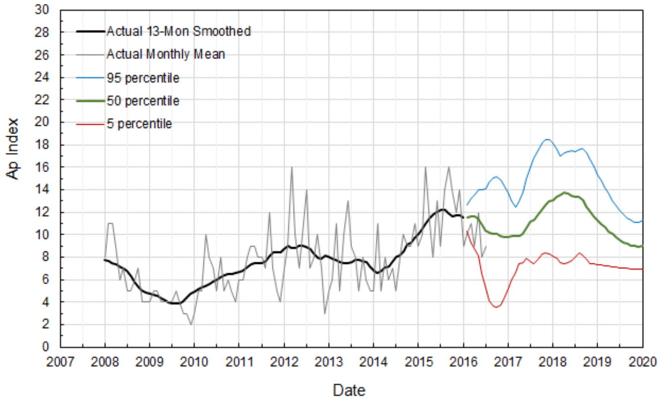
Figure 5. Recent Monthly Mean and 13-Month Smoothed Ap for Cycle 24
