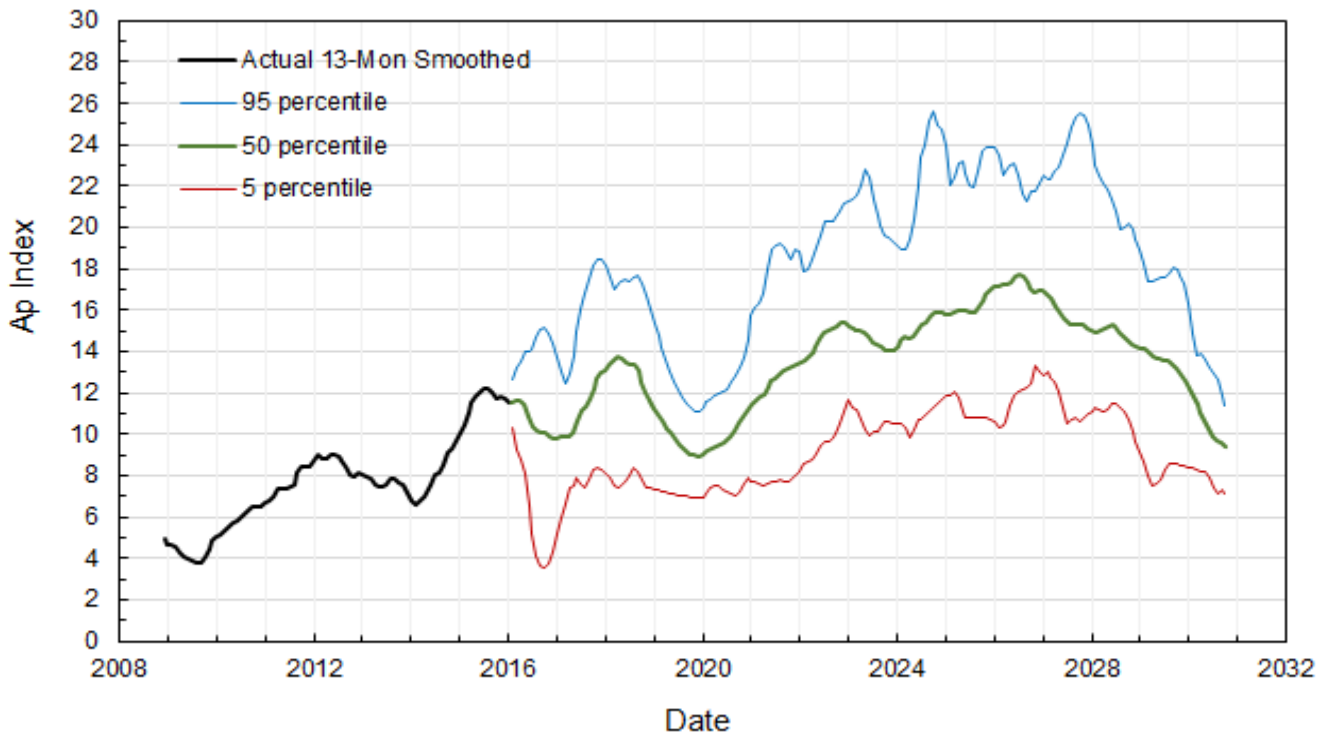
Figure 6. Estimate of 13-Month Smoothed Ap for Cycle 24* and Cycle 25
