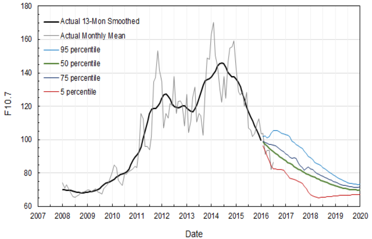
Figure 1. Recent Monthly Mean and 13-Month Smoothed Solar Flux for Cycle 24
