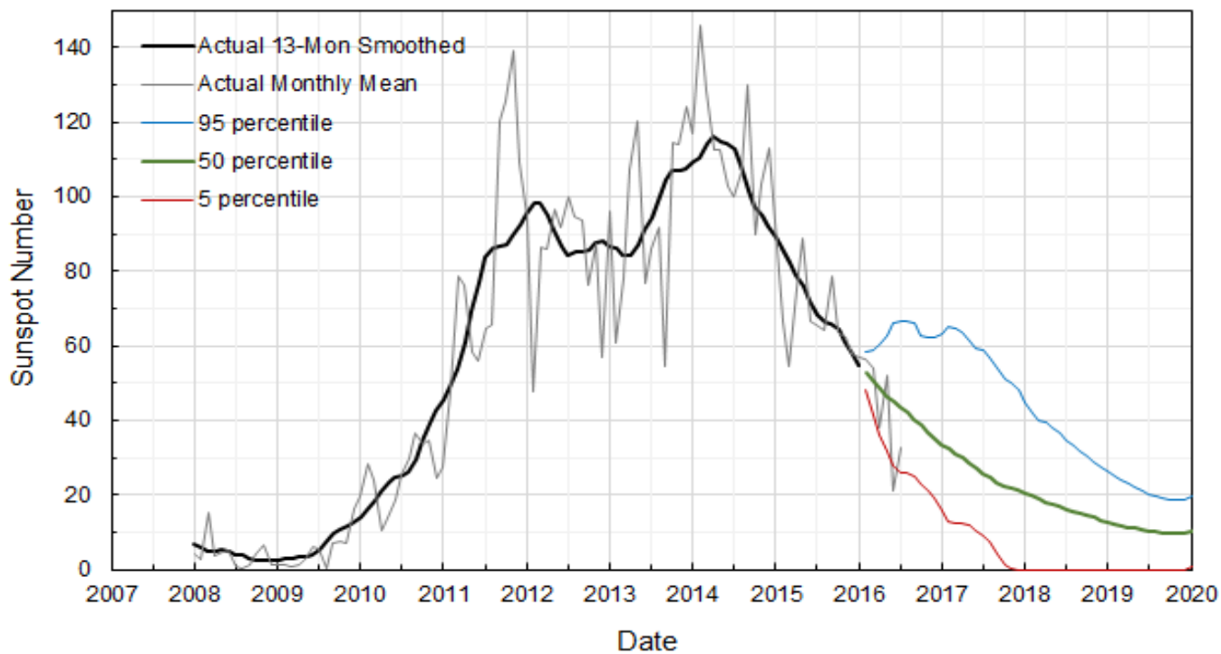
Figure 3. Recent Monthly Mean and 13-Month Smoothed Sunspot Number for Cycle 24
