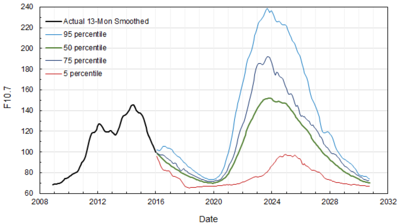
Figure 2. Estimate of 13-Month Smoothed Solar Flux for Cycle 24* and Cycle 25
