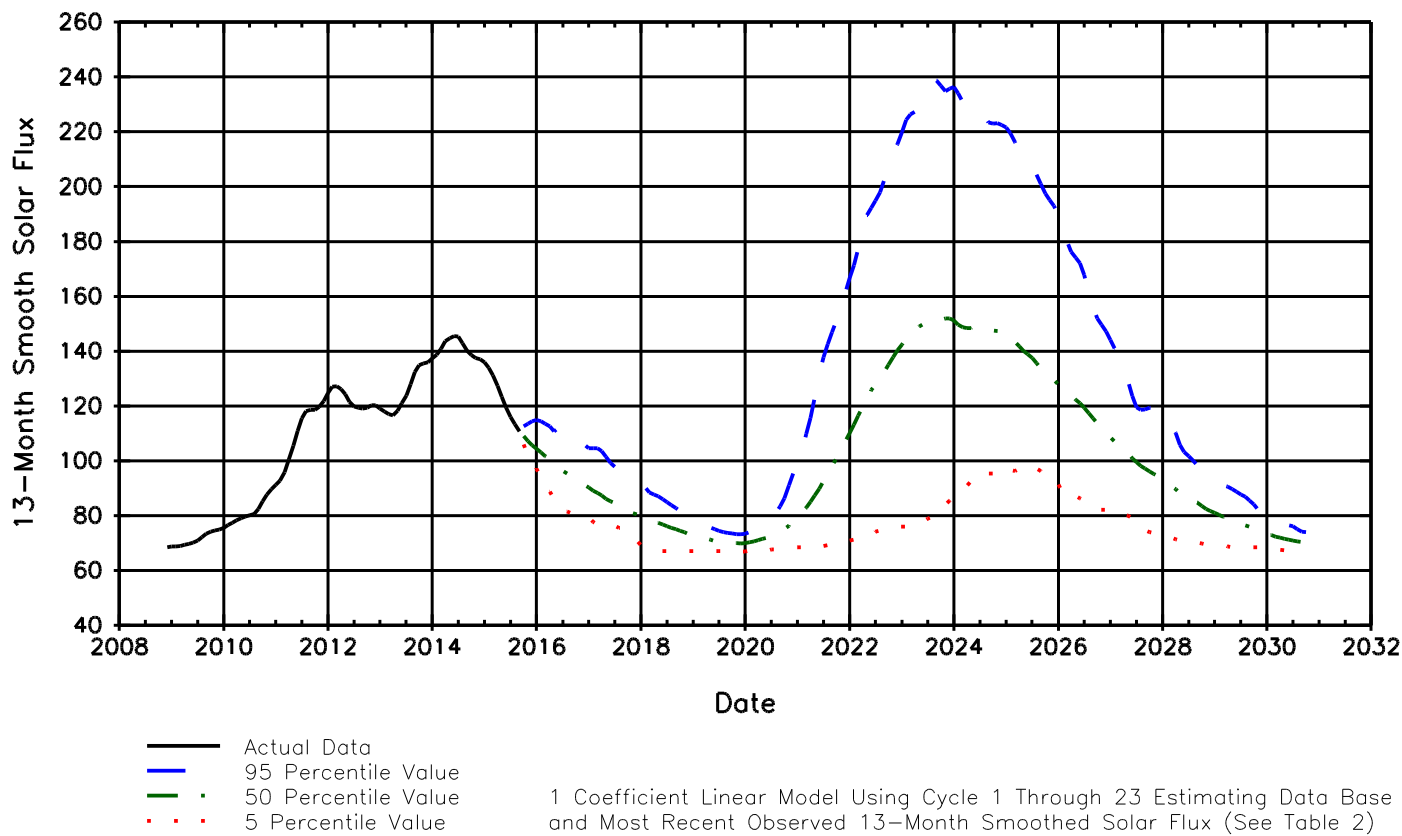
Figure 2. Estimate of 13-Month Smoothed Solar Flux For Cycle 24* and Cycle 25
