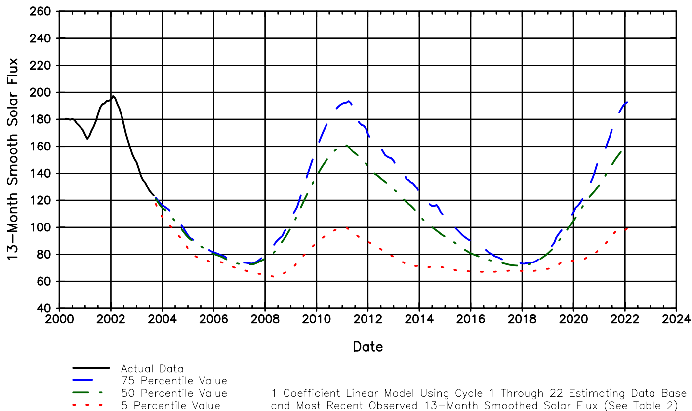
Figure 6. Estimate of 75 th Percentile 13-Month Smoothed Solar Flux For Cycle 23* and Cycle 24
