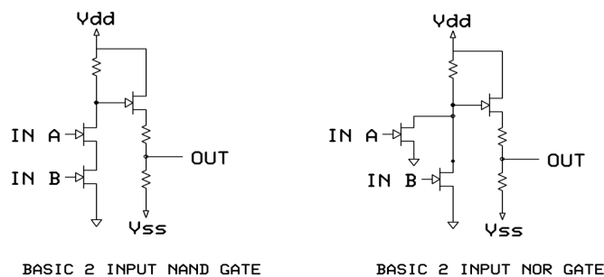
Figure 4.19.—SiC logic gate basics.
