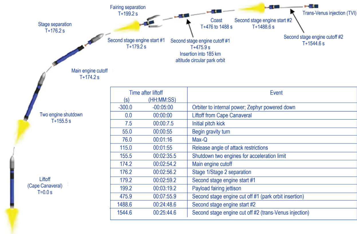
Figure 4.3.—Falcon 9 launch profile, trans-Venus insertion (TVI) and cruise phases.
