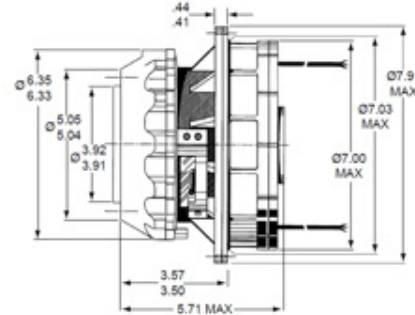
Figure 4.7.—Honeybee High Temperature Electric Motor and GE Test Article.
