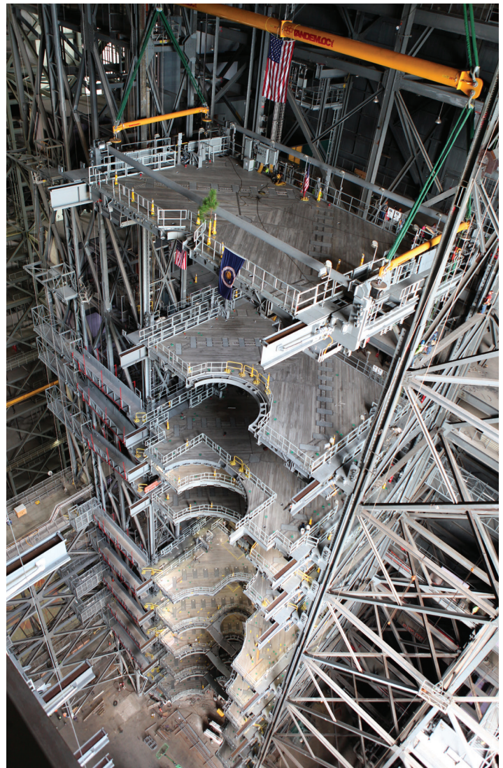
High up in the Vehicle Assembly Building at NASA's Kennedy Space Center in Florida, a crane lowers the final work platform, A north, for installation in High Bay 3 on Jan. 12, 2017. In view below are the nine previously installed levels of platforms. They will surround NASA's Space Launch System (SLS) rocket and the Orion spacecraft and allow access during processing for missions, including the first uncrewed flight test of Orion atop the SLS rocket. Photo credit: NASA/Frank Michaux
