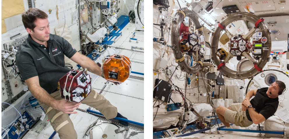
Figure 3: (left) SPHERES tether experiment—the thread between the two robots is too thin to make out in this photo. (right) The SPHERES RINGS payload.
