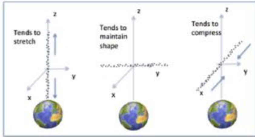
Figure 19: Effect of gravity gradient on linear cloud.
