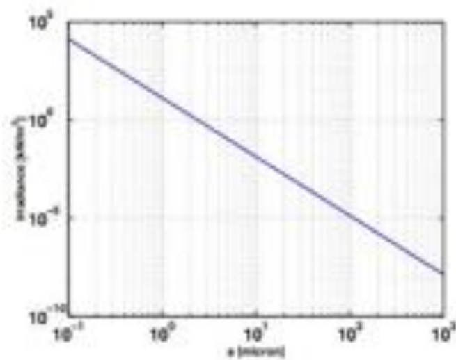
Figure 34: Laser irradiance vs. grain diameter.
