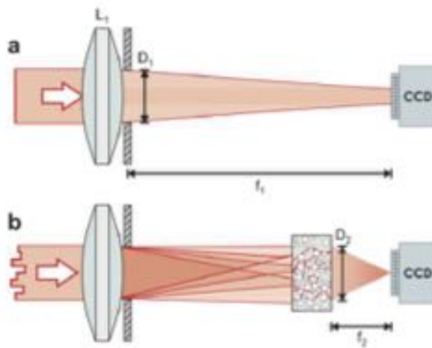
Figure 10: Disordered lenses: scattering in a medium behind a lens can be used to improve the focusing resolution to beyond the diffraction limit of that lens.
