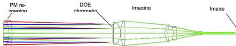
Figure 59: Diffractive Optical system chromatic corrector (courtesy M. Rud, JPL)
