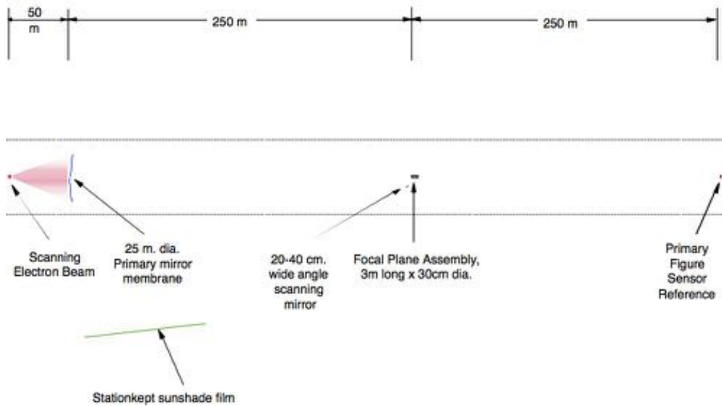
Figure 7: Adaptive structureless telescope proposed by I. Bekey .
