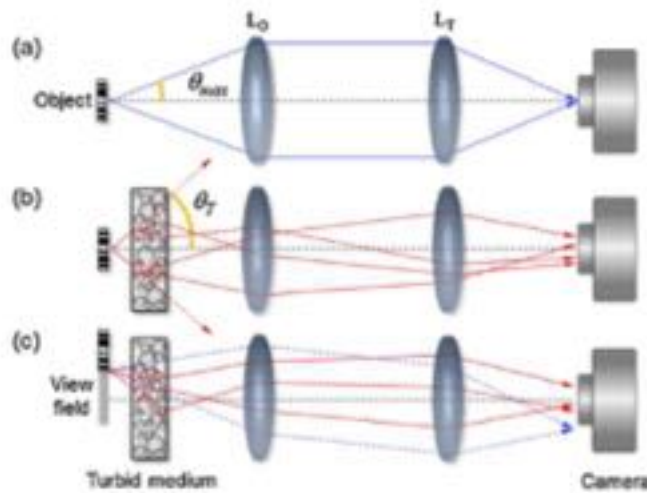
Figure 11: Turbid Lens Imaging: the turbid lens can perform wide-area imaging, rather than focusing a beam, with dramatically improved spatial resolution and an enlarged field of view.
