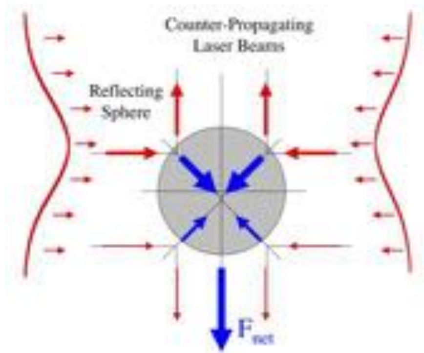
Figure 70: Counter-propagating laser beams incident upon a reflecting sphere produce a net repulsive force away from the beam.
