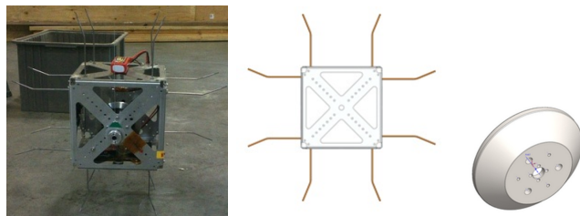
Figure 18: Prototype and CAD models (not to scale). The prototype, without the flywheel, has a mass of 1.39 kg and a moment of inertia about the axis of rotation of \approx 0.054 \text{ kg m}^2 . The flywheel is 0.57 kg and 8.07 \times 10^{-4} \text{ kg m}^2 .
