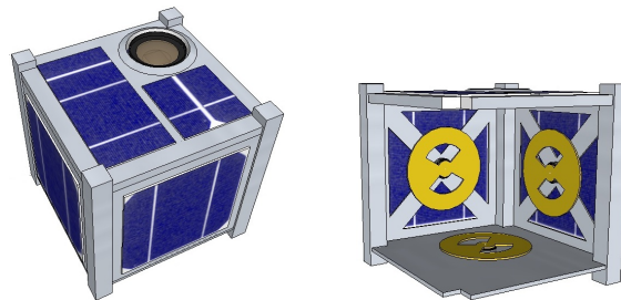
Figure 12: A spacecraft/rover hybrid is a planetary mobility platform sealed in one enclosure and actuated through three mutually orthogonal flywheels (for clarity, internal payload is not shown). By spinning the flywheels, one gives rise to surface reaction forces that make the rover tumble or hop. External spikes/feet (not shown here for clarity) are added to protect instruments and solar panels, and to improve traction. Trade-offs for spike design are discussed in Section 3.3.
