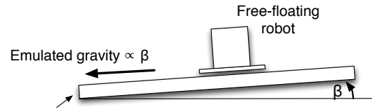
Figure 4: 3 DOF test stand on a frictionless table; by tilting the granite table, one can create a "small" force that emulates a low gravity field.
