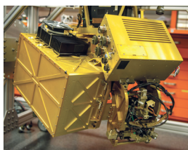
Principal Investigators Gerry Heymsfield and Lihua Li debuted their improved HIWRAP dual-frequency Doppler radar in the fall of 2013. (Photo Credit: Bill Hrybyk)
