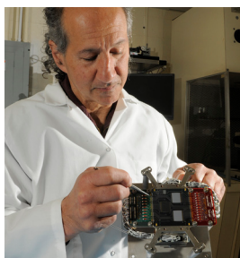
Murzy Jhabvala is shown here with the backup QWIP focal-plane assembly. (Photo Credit: Pat Izzo)
