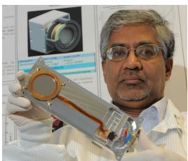
Scientist Shri Kanekal holds one of the solid-state detectors that will be used in the Compact Relativistic Electron and Proton Telescope slated to fly on a CubeSat. (Photo Credit: Pat Izzo)
