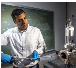
Technologist Vivek Dwivedi, who has distinguished himself as the go-to engineer for atomic layer deposition, has assembled a new reactor that he plans to use for thin-film experimentation. He is inserting the quartz crystal microbalance, one of the technologies included in his “virtual toothpick.” (Photo Credit: Bill Hrybyk)
