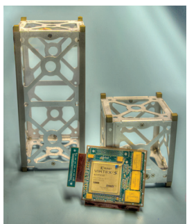
Shown here is the SpaceCube-Mini, along with two other devices that show the relative sizes of tiny satellites or CubeSats on which SpaceCube is slated to fly in the future. (Photo Credit: Bill Hrybyk)
