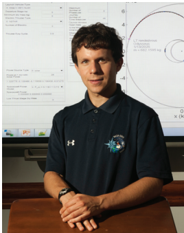
Jacob Englander has created an on-orbit determination tool that makes it faster to determine trajectories for spacecraft traveling to hard-to-reach destinations. The image projected in the background shows the trajectory to Odysseus, a Trojan asteroid. While not associated with any mission or mission proposal, Englander used his tool to create the design. (Photo Credit: Pat Izzo)
