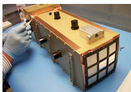
Three Goddard divisions successfully demonstrated NASA's first wide-field soft X-ray camera for studying "charge exchange."
