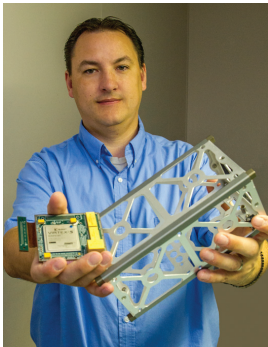
Engineer Gary Crum holds the SpaceCube-Mini, the smallest in a family of Goddard-developed onboard processors. The other device shows the relative size of a two-unit CubeSat, whose small size makes it the perfect platform for the SpaceCube-Mini. (Photo Credit: Bill Hrybyk)
