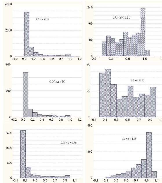
Figure 2. Histograms of the number of orbits N with different values of eccentricity e vs. perihelion distance q (in AU) for two types of near-parabolic orbits, elliptical (left column) and hyperbolic (right column).
