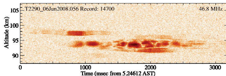
Figure 5. A likely “fossil” radar bolide event that has an \sim 3 sec lifetime. The progenitor event was not observed.
