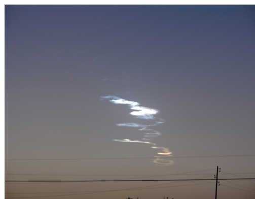
Figure 2. The trail of the July 23, 2008 fireball from Vose (Tajikistan). The photograph by M. Ahmetzyanov was taken at 14:58:58 UT
