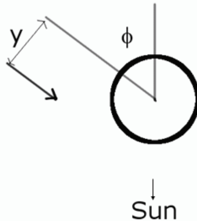
Figure 1. The angle \phi and the impact parameter y are defined as shown, in the heliocentric frame.
