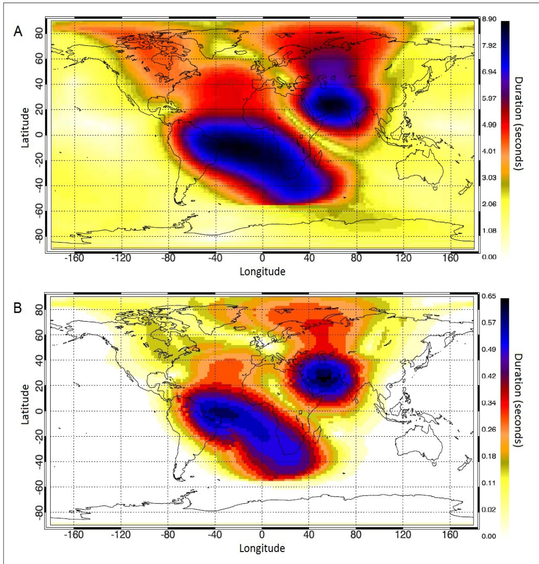
Figures 2. (a) A global simulation of the duration of meteor trail turbulence of a single 1 \mu\text{g} meter simulated across the world traveling a 55 \text{ km/s} at 00:00 UT on January 1 st . The units of the color bar are in seconds after meteor trail creation. Each pixel results from the measured duration of a simulation of the type shown in Figure 1a. The location of the meteor presented in Figure 1 is denoted by a (*) near North Carolina. Figure 2a illustrates the effect that the atmospheric properties electron density and horizontal wind speed have on a meteor's trail duration. (b) A global simulation of the duration of meteor trail turbulence of a single 0.1 \mu\text{g} meter simulated across the world traveling a 55 \text{ km/s} at 00:00 UT on January 1 st . The units of the color bar are in seconds after meteor trail creation. Each pixel results from the measured duration of a simulation of the type shown in Figure 1a. Notice that a meteor of lesser mass meteor experiencing the identical atmosphere as Figure 2a will produce meteor trails of shorter duration or no meteor trail at all depending on the location.
