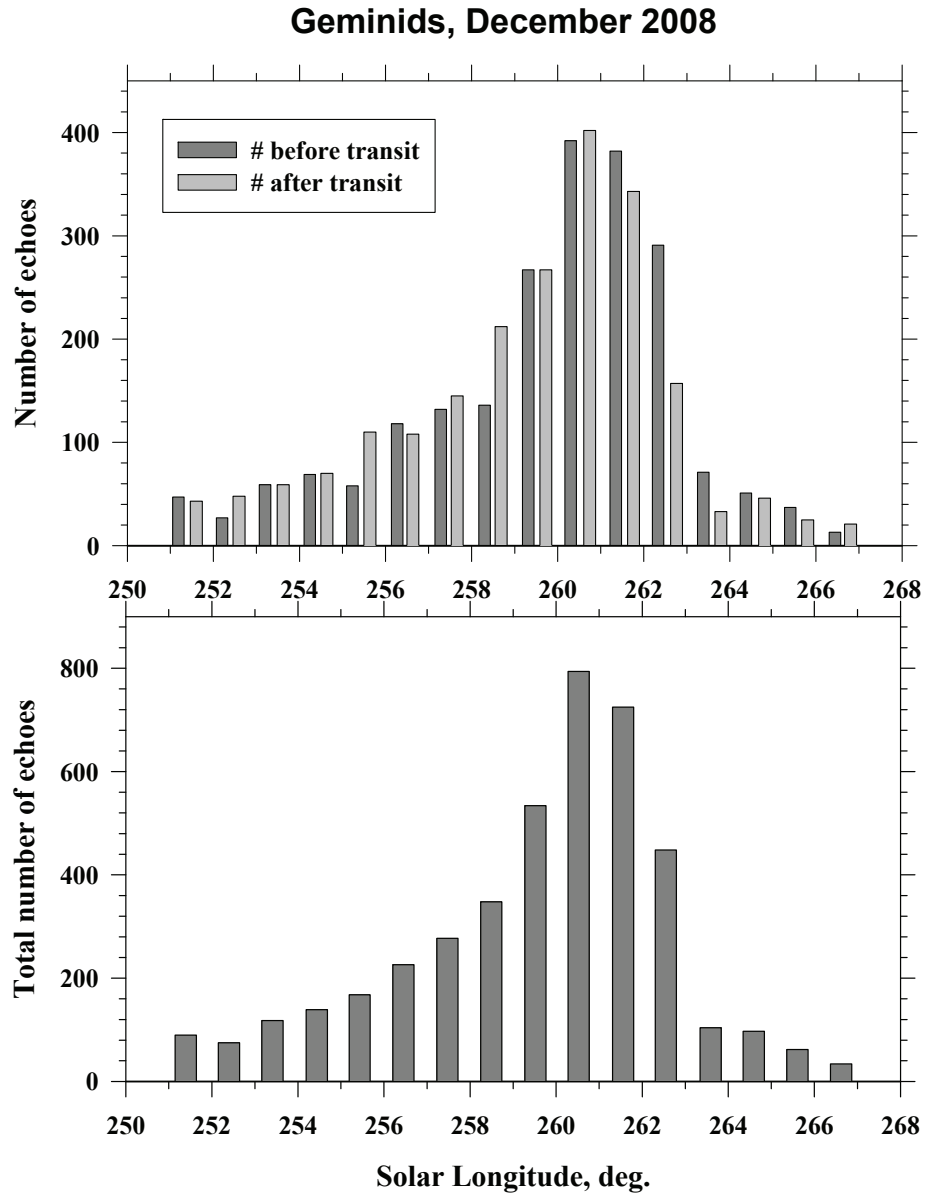
Figure 7. The echo rate seen by the radar over the period of significant activity; the rate before and after transit (top) and the total rate for each night (bottom).
