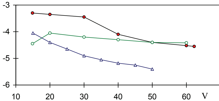
Figure 2. Variation of mean values of \lg I_p/q as a function of velocity V .
