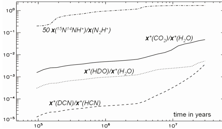
Figure 2. Time dependency of the nitrogen isotope ratio in the gas phase (note the factor of 50 to present all curves in the same figure), the D/H ratios in the ice phase and the CO_2/H_2O ratio for the polar to non-polar ice fraction calculated for the slowly evolving quasi-stationary prestellar core.
