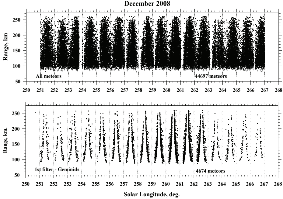
Figure 3. Total observed meteor echoes over the period 251^\circ to 267^\circ in S.L. in 2008 (top) and those extracted by the 1 st filter (bottom).
