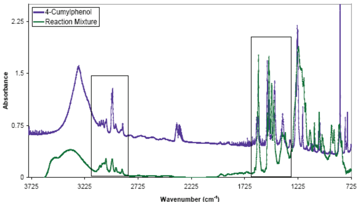
Figure 3. Comparison of 4-cumylphenol IR spectrum (upper curve) with that of the reaction mixture (lower curve). This reaction mixture was 70wt% sulfuric acid heated to 40°C for 5 minutes and then remained at 20°C for one day. 4-cumylphenol is an analog for the predicted product, 4-(1-phenylethyl) phenol, shown in Figure 2.
