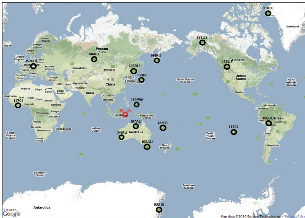
Figure 2. A global map (courtesy of CTBTO, web: http://www.ctbto.org ) showing all stations (black circles) that detected the Indonesian bolide event circled in red.
