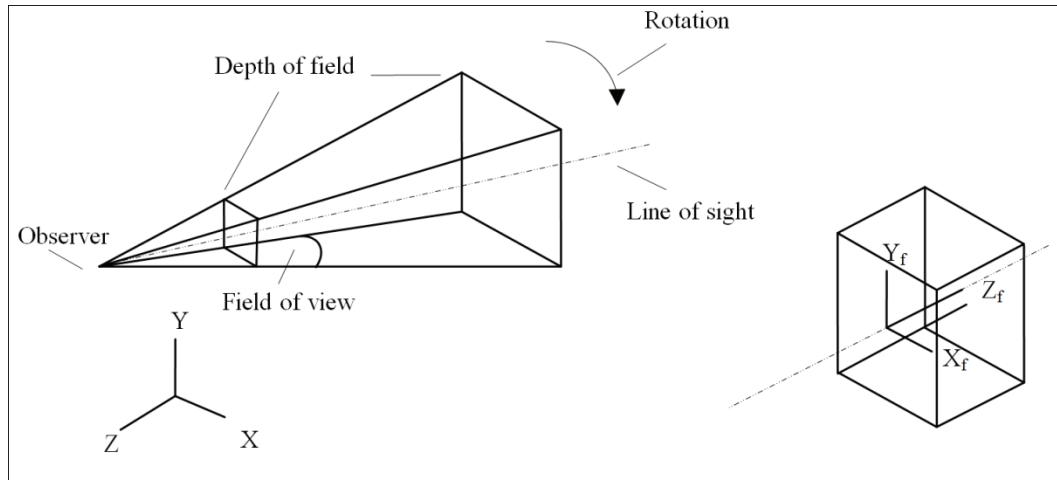
Figure 7. An image frustum in heliocentric space, and the rectangular frustum space. Any astronomical image is a representation of the three dimensional frustum volume defined by the observer location, the field and depth of view of the image, the line of sight, and the rotation of the image. Points in heliocentric space may be easily transformed into points in the frustum space, facilitating image-object intersection and object motion characterization.
