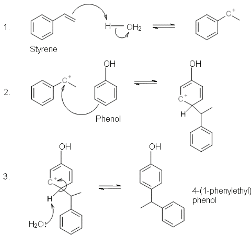
Figure 2. Theoretical acid-catalyzed reaction between phenol and styrene yields 4-(1phenylethyl) phenol. Note loss of =\text{CH}_2 in step 1 and addition of -\text{CH}_3 group.
