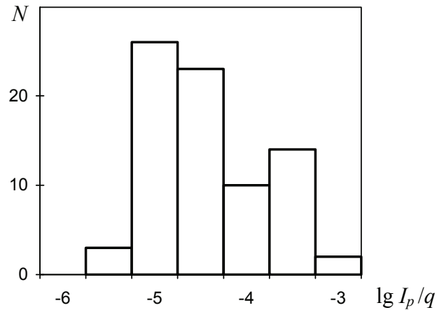
Figure 1. Observed distributions of ratio \lg I_p / q .
