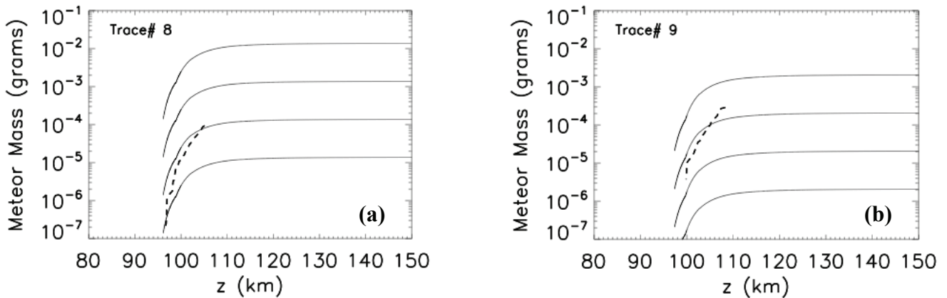
Figures 4. (a) Here the solid curves are the inertial masses (for trace #8) computed with the numerical model, using the best-fit value of mp_s^2 together with four different assumed values of the meteor density \rho_s , namely (from top to bottom) 0.1, 0.316, 1.0 and 3.16 g/cm 3 . The dashed curve is the “mass1” (mass determined from the measured cross sections together with the electrostatic scattering model). (b) Same as for (a), but representing trace #9.
