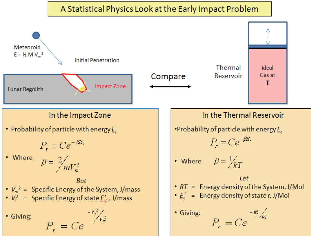
Figure 8. With hypervelocity impacts into particulate regolith, the impact specific energy is rapidly thermalised leading to a statistical physics approach. The specific energy of the impact is an exact analog of the canonical energy density of a thermal system leading to a canonical expression of the probability of a particle being in any particular energy state.
