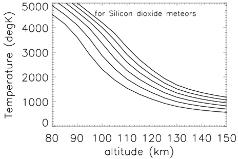
Figure B1a. Composite plots of steady-state temperatures vs altitude for \text{SiO}_2 meteors with velocities of 30, 40, 50, 60, 70 and 80 km/s (in that order from bottom to top).
