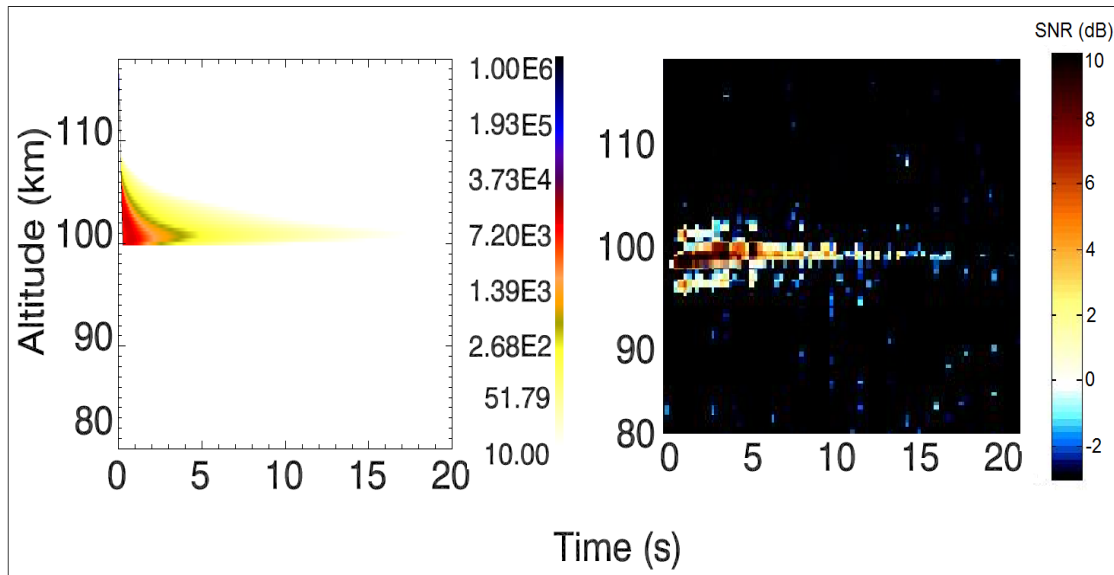
Figure 1a. A simulated RTI simulation for a meteoroid near North Carolina compared to an observed meteoroid in North Carolina (Latitude = -35^\circ and Longitude = -55^\circ ) conditions for 00:00 UT, on June 27th. The simulated meteoroid mass is 10 \mu\text{g} , traveling at a velocity of 70 \text{ km/s} , composed of an atomic mass of 30 \text{ AMU} . The duration of the trail turbulence is approximately 15 seconds. The color bar shows instability growth rate in \text{s}^{-1} for the trail, and the simulated head echo displays electron line density per meter divided by 10^6 (units chosen such that they appear on the same scale).
