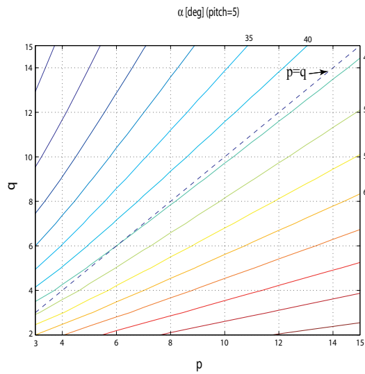
Figure E.20: Contour plot of angle of bar \alpha [deg] ( L/D = 3 )
