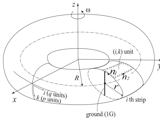
Figure B.1: Tensegrity torus
