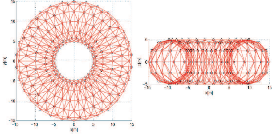
Figure A.7: Torus with dominant members
