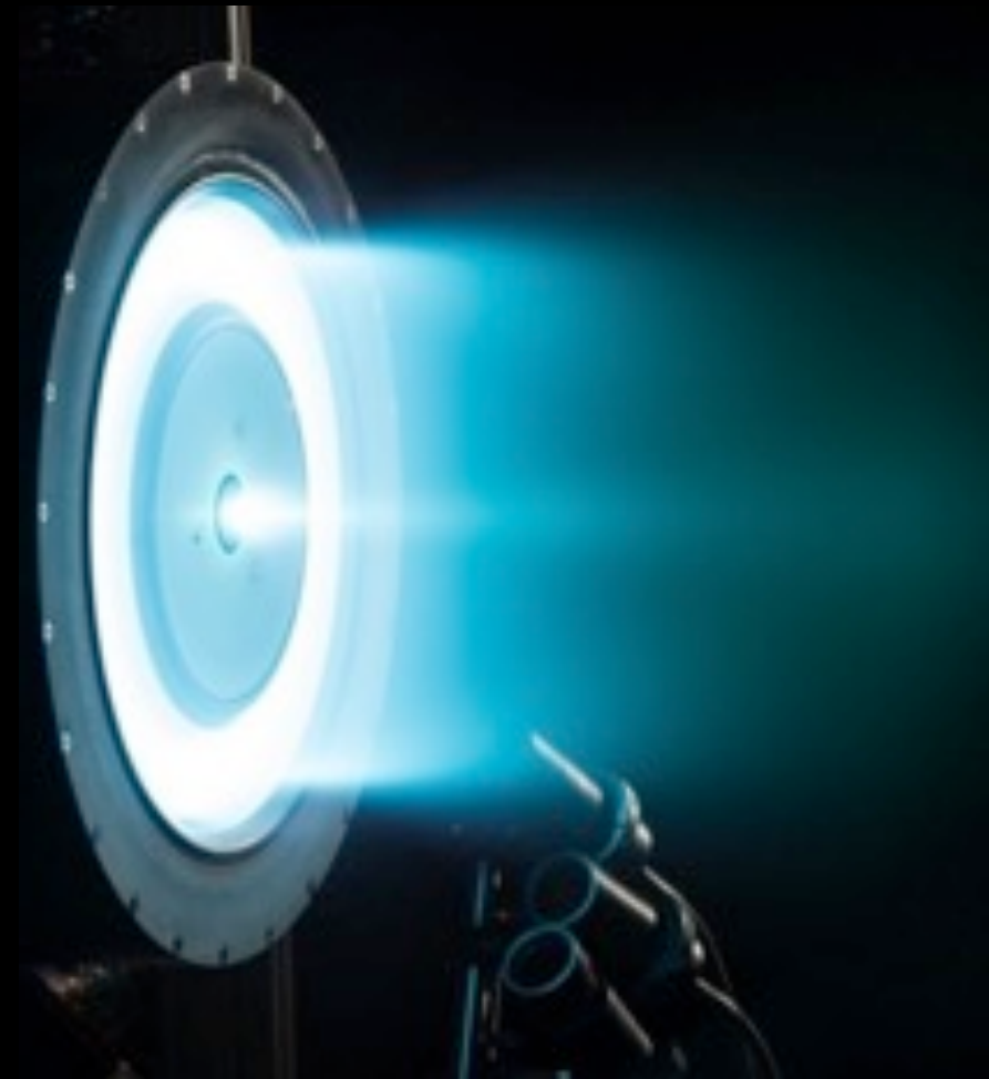
12.5 kW, 3,000 s hot-fire thruster test at GRC
