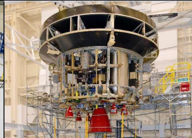
European Service Module Structural Test Article (ESM STA) at Glenn Research Center Plum Brook Station in Ohio
