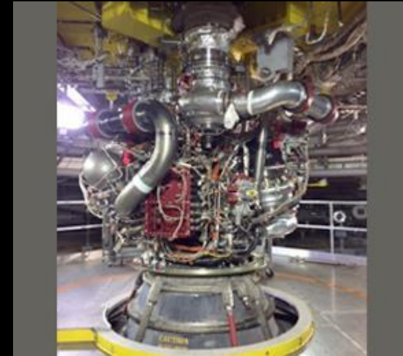
RS 25 flight engine 2059 installed for testing at Stennis Space Center
