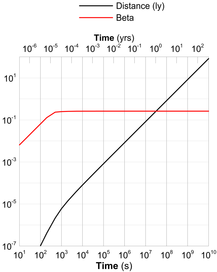
Figure 25 – WaferSat case with same DE-STAR 4 driver (70 GW – 10 km array) as in Fig 20 but for wafer scale spacecraft driven by 1 meter sized reflector (1 micron thick), Wafer mass is 1 g and reflector mass is 1.4 g. Total mass is 2.4g. Parameters shown are relativistic factor beta and distance vs time. Note that Alpha Centauri (4.3 ly) is achieved in about 20 years with 10 ly achieved in about 45 years.
