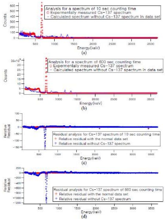
Figure 3.14. MP_PIM analysis of Cs-137 measured spectra without the Cs-137 computed spectrum in the data set (a) for 10 sec counting time, and (b) for the 600 sec counting time and relative residuals (c) for 10 sec counting time, and (d) for the 600 sec.
