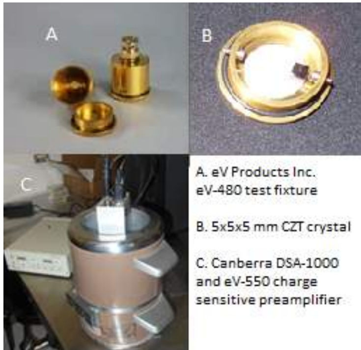
Figure II.5. Equipment setup for spectrometer grade 5 mm 3 planar CZT crystal from eV Products Inc.
