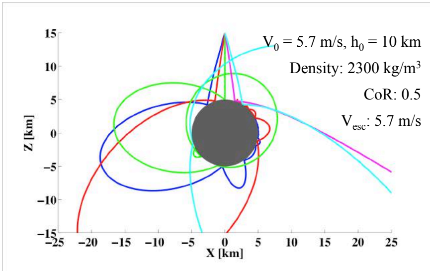
Figure III.14. Lander rebound trajectories on 10 km asteroid, v_0 = 5.7 \text{ m/s}
