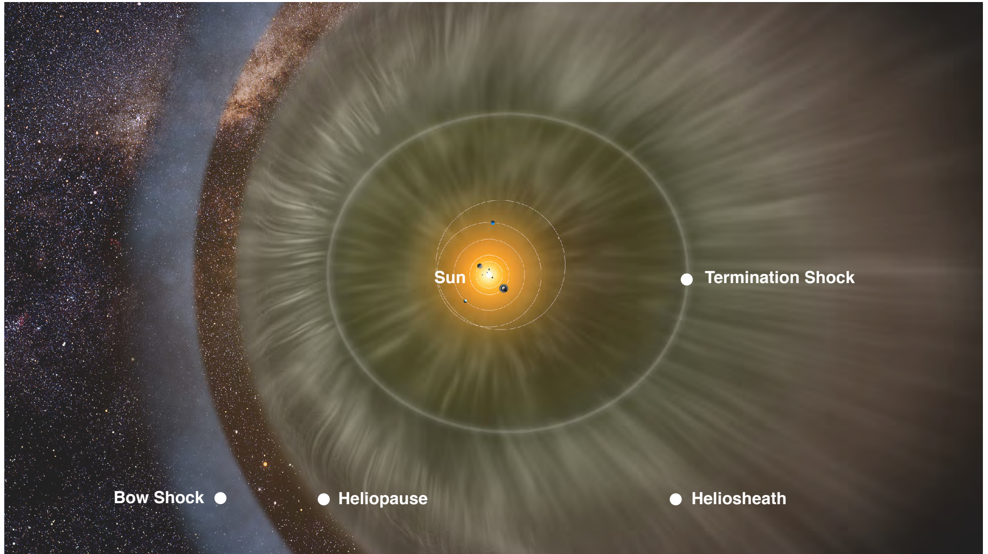
The Heliosphere
