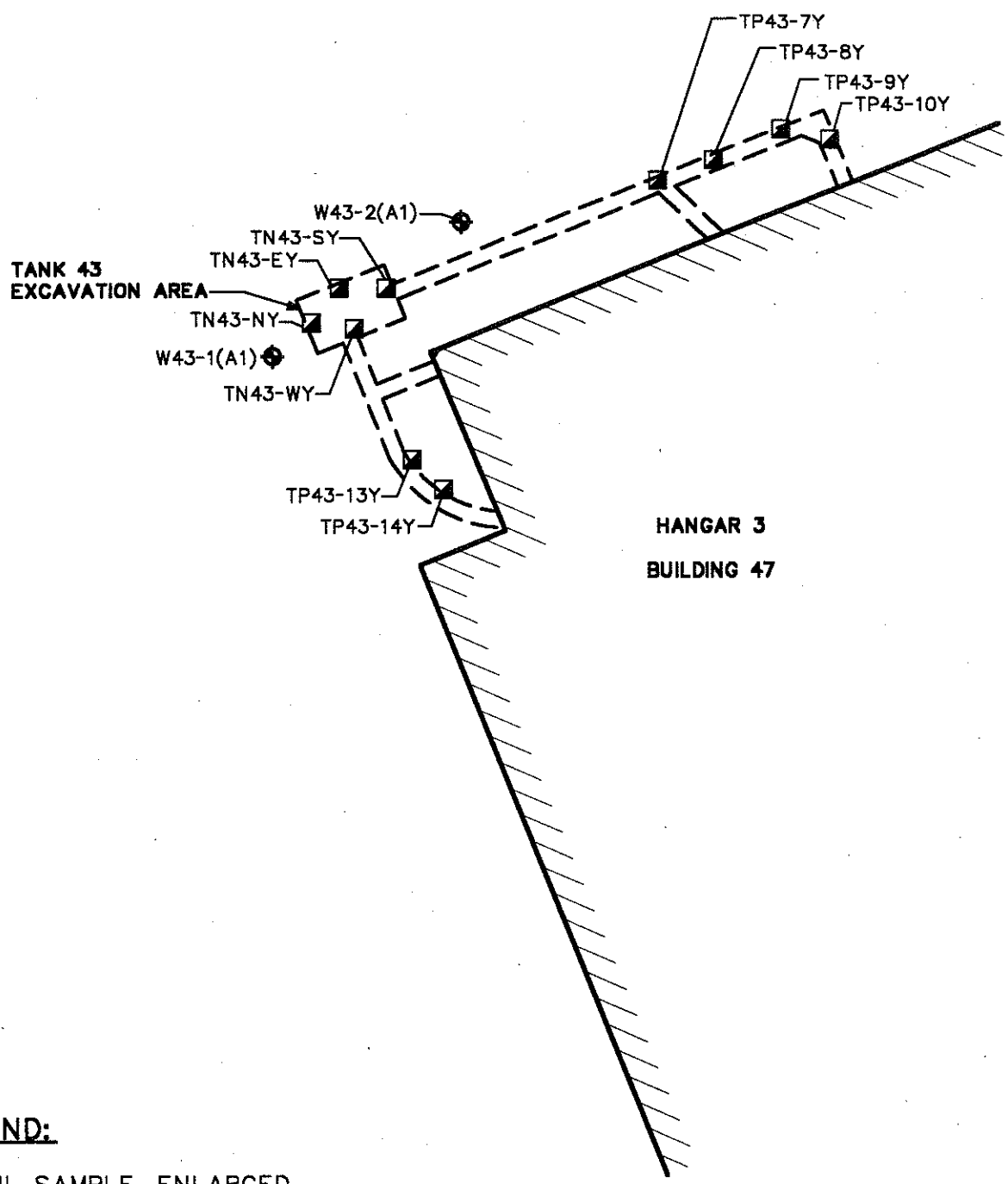
FIGURE 13 NAS MOFFETT FIELD SITE 19 - TANK 43 EXCAVATION AND SAMPLE LOCATIONS
