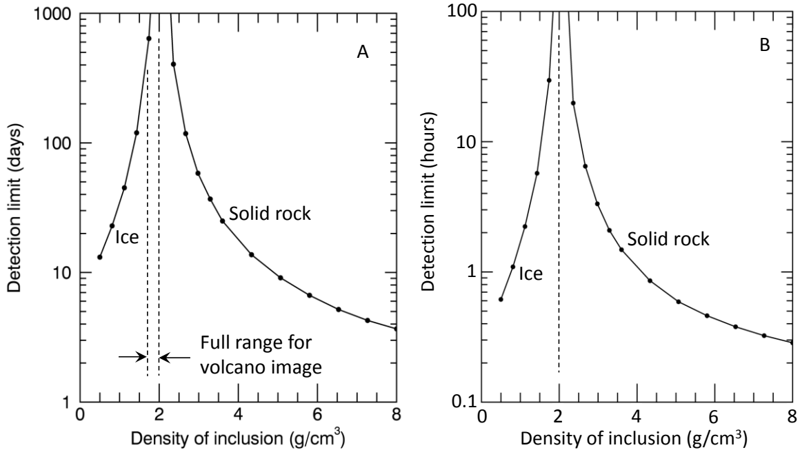
Figure 13. Detection limit for an inclusion within a small body (asteroid or comet) as a function of inclusion density. The density of the outer portion of the asteroid is 2 \text{ g/cm}^3 . Case A is for prompt muons ( > 0.1 \text{ TeV} ) produced in an 800-m diameter asteroid with a 400-m diameter inclusion. Case B is for muons ( > 10 \text{ GeV} ) produced by the decay of pions and kaons in a 50-m diameter asteroid with a 20-m diameter inclusion. The full range of densities in the volcano image of Fig. 2 is shown for comparison (left).
