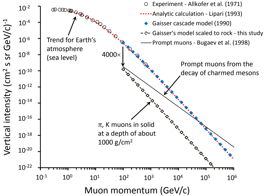
Figure 7. The Gaisser cascade model of the vertical muon flux at sea level on Earth is scaled to a solid with a density of 1.6 g/cm 3 , typical of planetary regolith materials. Muon production in the top layer of an asteroid by the decay of pions and kaons is over three orders of magnitude less than in Earth's atmosphere. A prompt component from the decay of charmed mesons does not depend on density.
