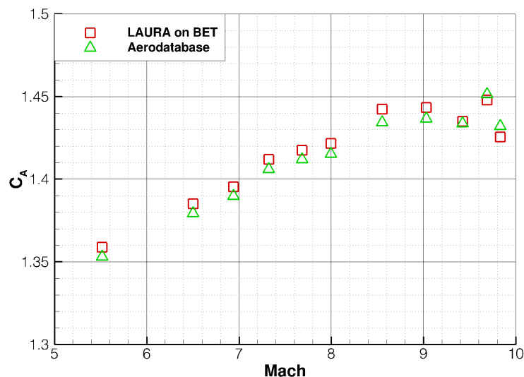
LAURA Aerodynamics on IRVE-3 BET Compared to Pre-Flight Aerodatabase
