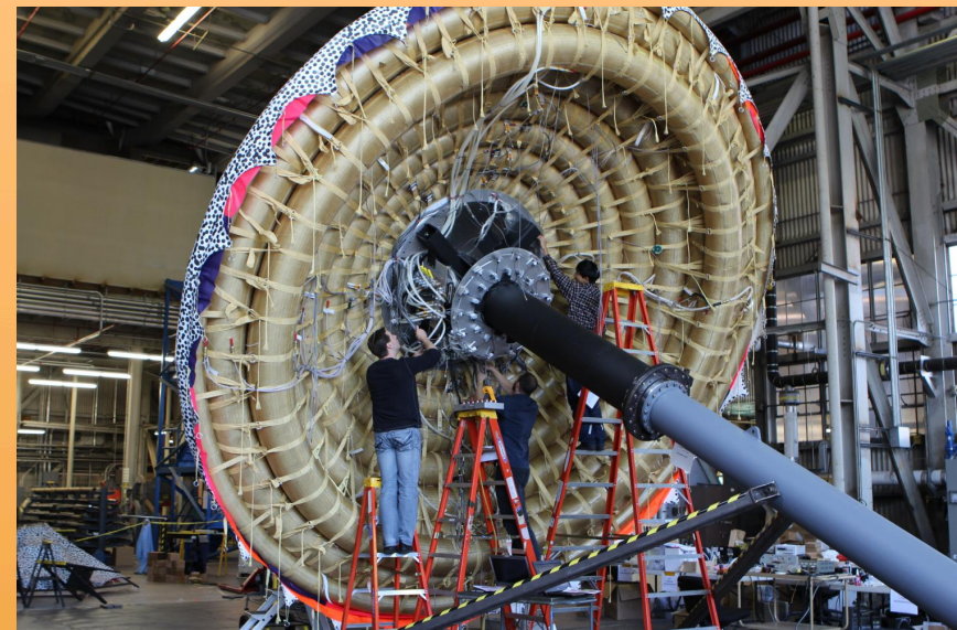
Installation in 40 x 80 ft Test Section
