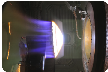
IRVE-3 Nose Cap Test TP2 – 2011
