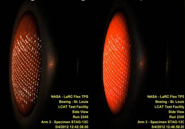
Boeing LCAT Stagnation Test (50 W/cm 2 )
