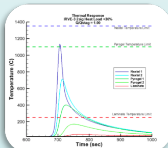
TPS Modeling
