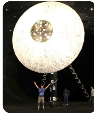
Aero Load/Deflection Test 6 m Dia (NFAC-2012)
