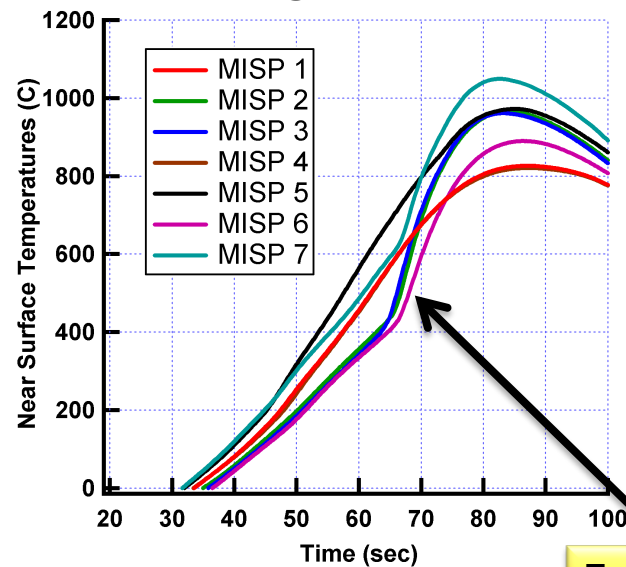
Top TC data @ each MISP location
