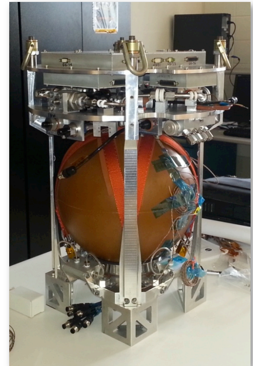
IRVE-4 Inflation System (ready for avionics integration)
