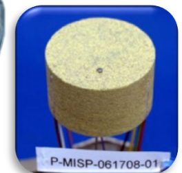
MEDLI Instrumented Sensor Plug (MISP)
