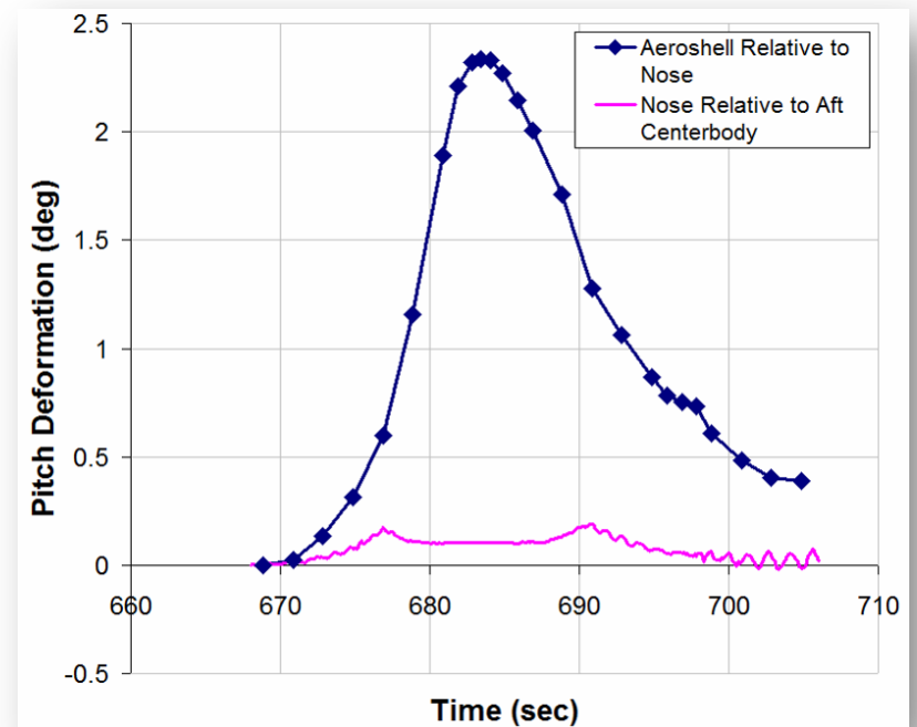
Observed Deflections
