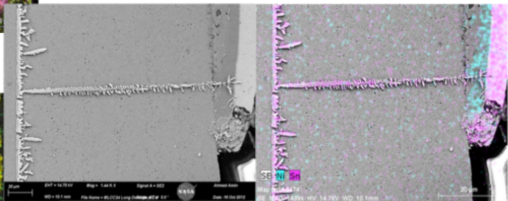
Fig. 10: Sn Dendrite Growth from Substrate 0.8V WLT
