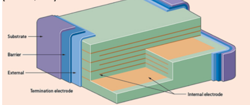
Fig 1: Typical construction of a ceramic capacitor
