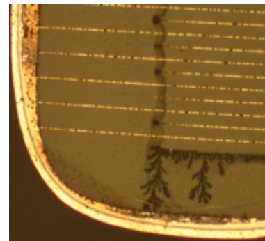
Fig. 3: Dendrite Growth
