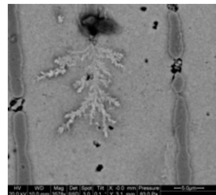
Fig. 6: Silver Dendrite (1.3V, 25°C/85% RH)
