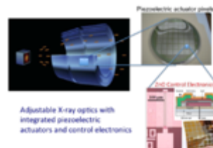
Fig. 1: Grazing incidence optics with piezoelectric actuation and integrated control electronics
