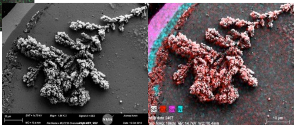
Fig. 12: Cu Dendrite Growth from External Layer in Termination, 1.3V WLT (Thick Moisture Layer)
