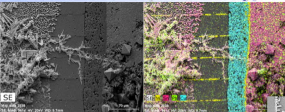
Fig. 9: Pb/Sn Solder Mixture Forming Dendrite Growth, 1.3V WLT
