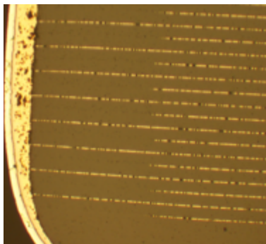
Fig. 2: Capacitor Pre-Test
