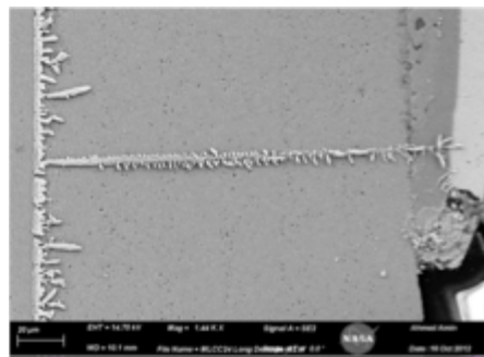
Fig. 4: Tin Dendrite (BME 0.8V WLT, 95 mins)
