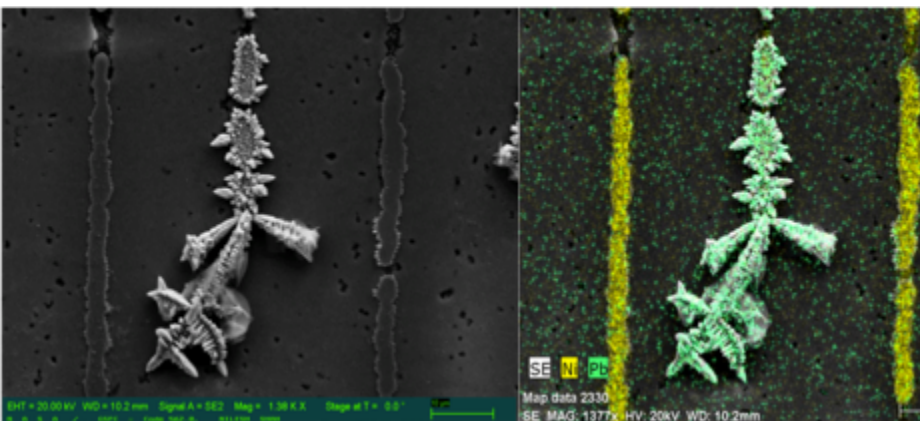
Fig. 11: Pb Dendrite Growth from Substrate, 1.3V WLT
