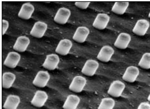
Magnification of a sample of an aluminum-indium alloy. When the sample is melted then controllably solidifies in the AGHF; the indium forms in cylindrical fibers within a solid aluminum matrix.
