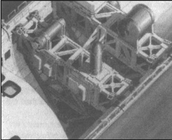
USMP experiments are mounted on Mission Peculiar Equipment Support Structures in the Shuttle Cargo Bay.
