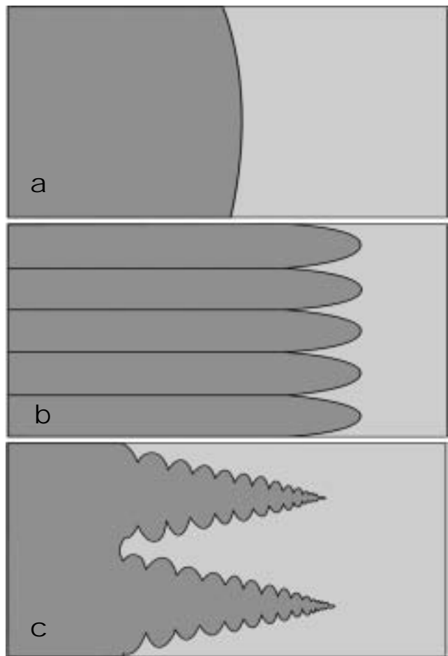
Representations of different shapes of the liquid-solid interface in a solidifying material: a) planar; b) cellular; and c) dendritic. More information about interface morphology is provided in the Metals and Alloys discussion in the Materials Science section of this publication.
