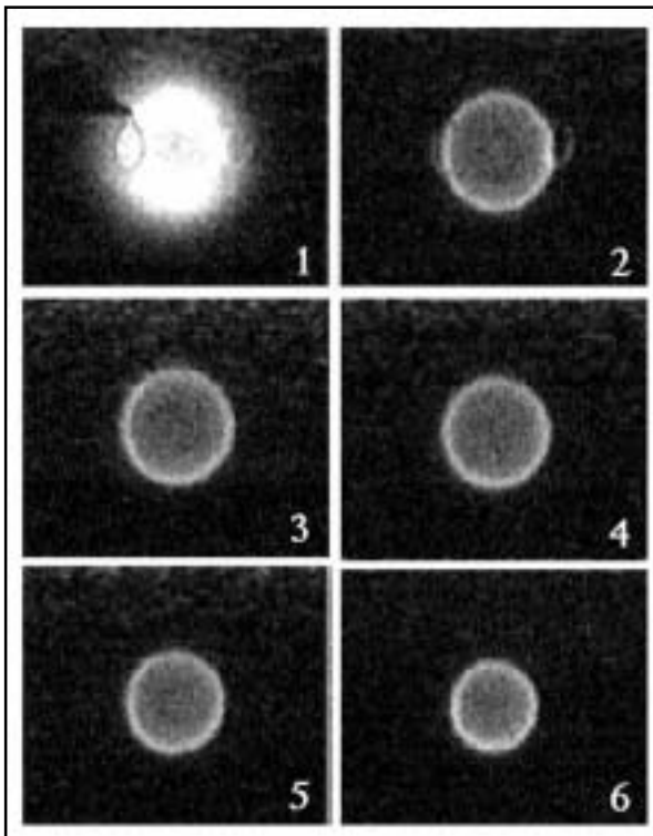
Ultraviolet images of OH radiation taken at half-second intervals during a drop tower test of the Droplet Combustion Experiment. The diameter of the flame produced by burning a heptane droplet decreases in freefall.
