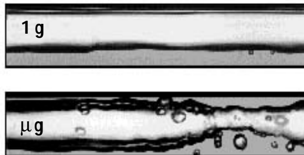
Side views of water and air flowing through a clear pipe. At 1g, the air stays on top. In microgravity, the air can form a core down the center of the pipe.
