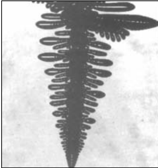
A dendrite grown in the Isothermal Dendritic Growth Experiment aboard the USMP-2. This is an example of how most metals solidify.
