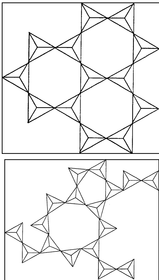
Schematic of silicon dioxide tetrahedra. The top view is of a crystalline ordered structure. The bottom view is of a disordered glassy solid.
