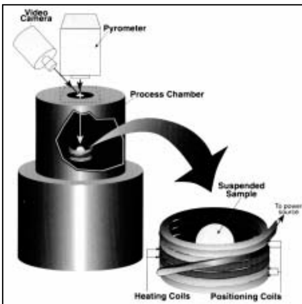
Schematic of the Electromagnetic Containerless Processing Facility (TEMPUS) used on Shuttle missions STS-65 and STS-83.
