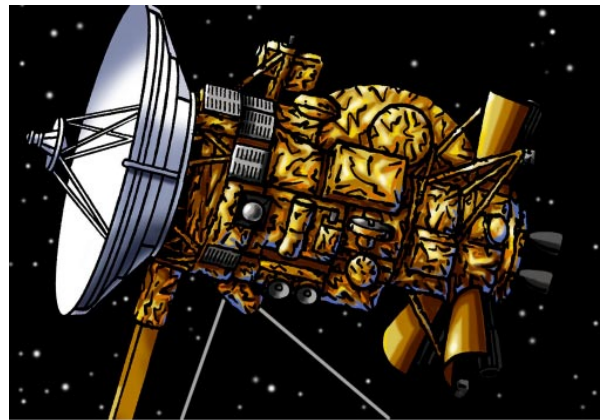
Cassini-Huygens Spacecraft
