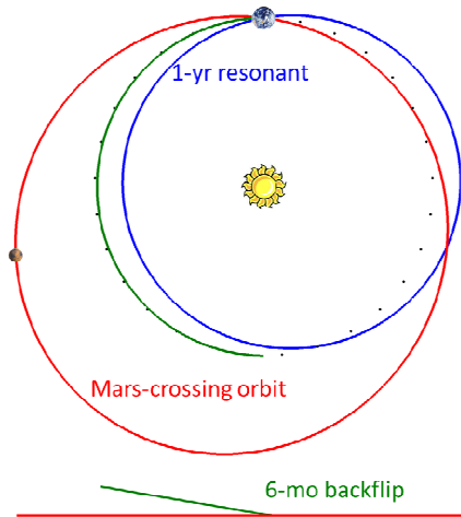
Figure 3. Redirecting small asteroids to Earth flybys could enable a wide variety of orbits where the asteroid could be “stored” including Earth-resonant orbits and Mars-crossing orbits.
