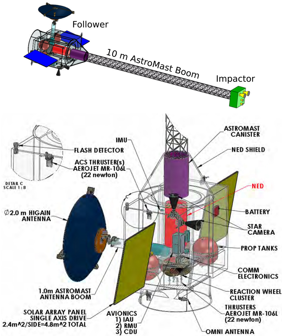
Figure 9: An experimental HAIV flight system designed by the MDL of NASA GSFC [15].
