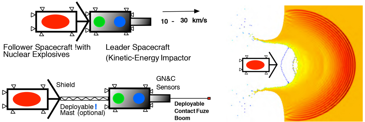
Figure 2: Initial conceptual illustration of a two-body hypervelocity asteroid intercept vehicle (HAIV) system, which was proposed for a NIAC Phase 1 Study in 2011 [12].
