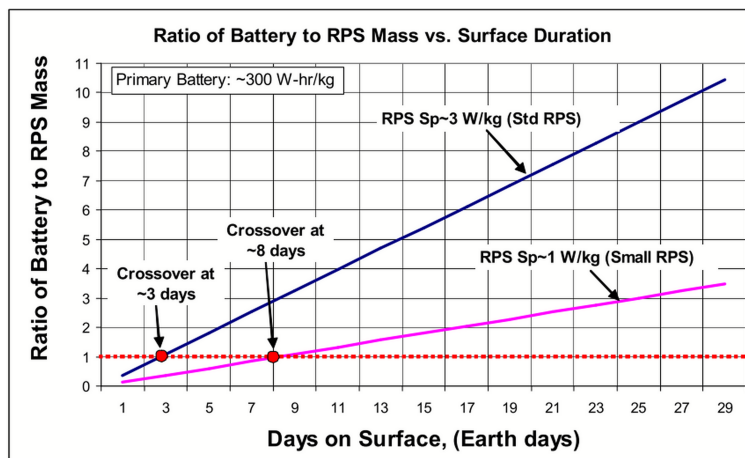
Figure 7.1: From 2006 mission architecture study [18]. Radioisotope power is preferable to battery power for a European lander.
