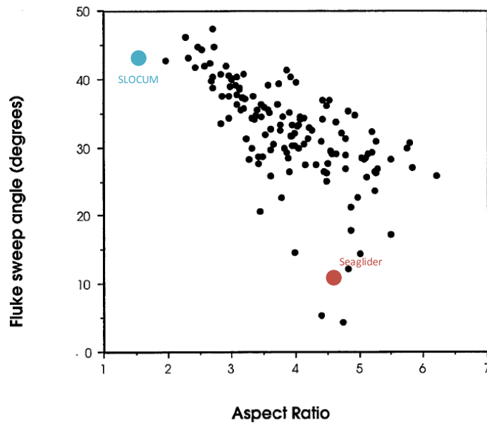
Figure 6.7: Relationship between sweep angle and aspect ratio of the tail fin of marine mammals. The corresponding values for Seaglider*[10] and SLOCUM [8] are included. Original figure from Review of Dolphin Hydrodynamics and Swimming Performance by Frank E Fish [9]. *Estimated from photograph.
