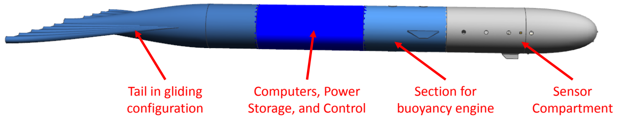
(a) Hydrobot in gliding configuration
