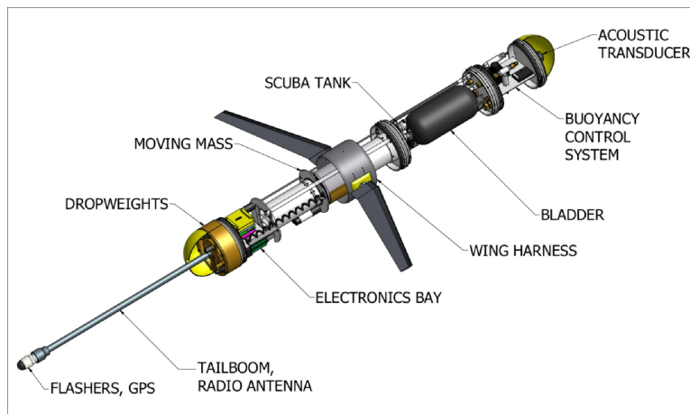
Figure 6.2: Annotated schematic of the Virginia Tech underwater glider [4].
