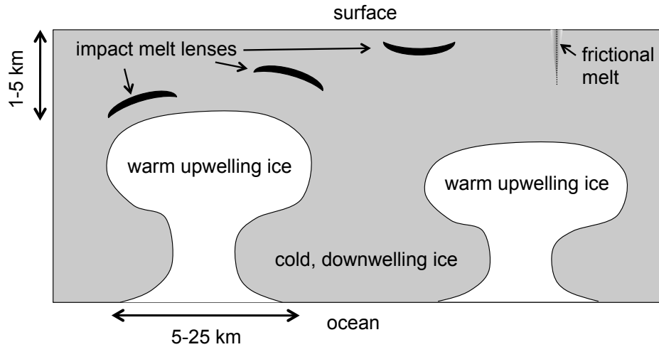
Figure 2.2: An illustration of possible structures in the ice shell (after [2]). Warm upwellings and cold downwellings with scales of about 10 km result in lateral temperature variations of about 10 degrees C. Near the surface, re-freezing of impact- or friction-generated melts may leave lenses or sheets of precipitated salts. In warmer regions these may remain liquid as hyper-saline brines.
