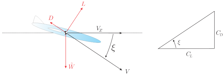
Figure 6.1: Free body diagram for wings-level gliding flight [3].
