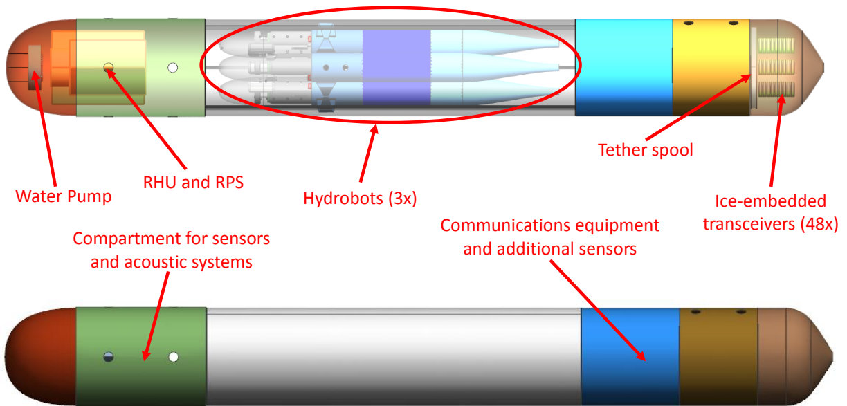
Figure 9.2: Notional design of surface unit with cryobot in its stored configuration.
