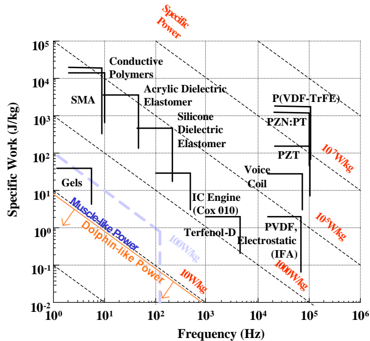
Figure 6.8: The specific energies and operating frequencies of several smart materials [11]. The diagonal lines indicate specific powers, which are the product of the specific energy and frequency. The region corresponding to dolphin-like specific power is indicated by the orange line. These specific powers are based on the total mass of the animal, so is likely less than the propulsive specific power[9].
