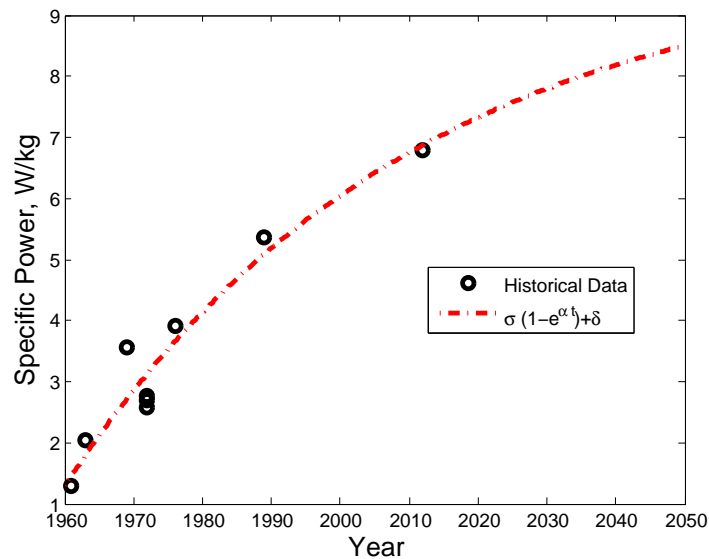
Figure 6.12: Specific Power of RTGs over time with an exponential fit. Historical data per [14]; ASRG data per [15].
