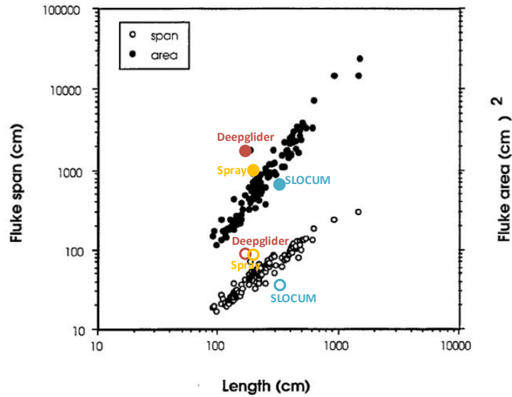
Figure 6.6: Comparison of the relation of tail fin span and area with the body length of various marine mammals (primarily dolphins). The corresponding values for Deepglider [6], Spray Glider [7], and SLOCUM [8] are included. Original figure from Review of Dolphin Hydrodynamics and Swimming Performance by Frank E Fish [9].
