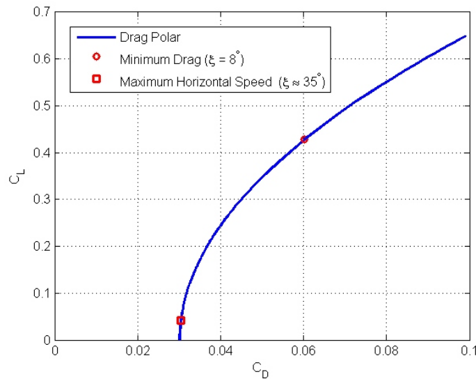
Figure 6.4: Drag polar for a model of the Slocum glider [3].
