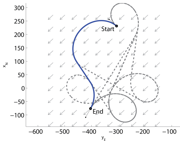
Figure 6.5: Example of vehicle path optimization in a steady, uniform flow [5].
