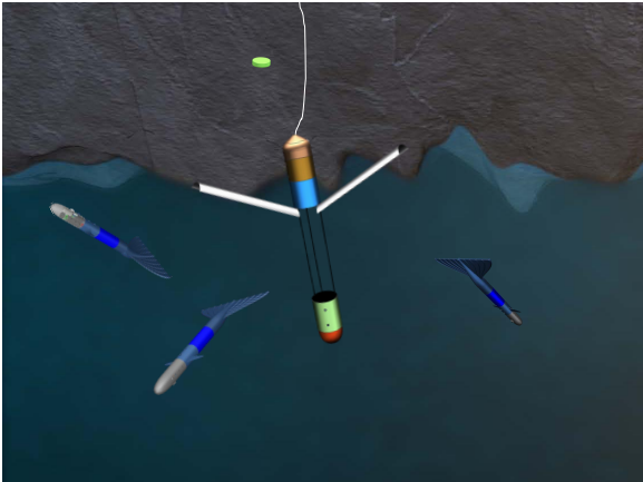
(a) Cryobot embedded in ice with deployed hydrobots
