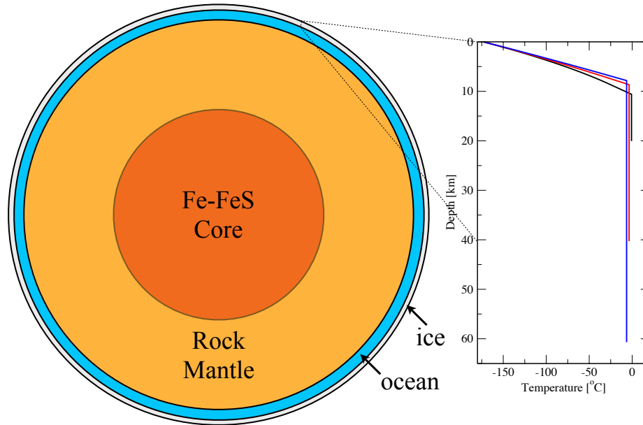
Figure 2.1: Europa’s interior structure (left) consisting of a metallic core, rock mantle, and water/ice shell [1]. The equilibrium temperature structure of the ice shell is shown on the right, for three different shell thicknesses: 20 km (black), 40 km (red), and 60 km (blue).
