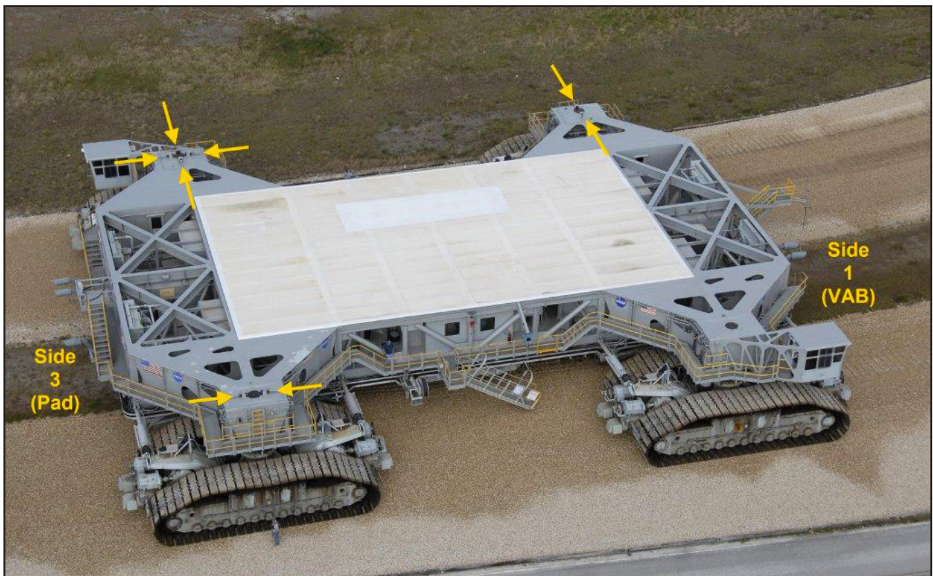
An aerial view of crawler-transporter 2 showing the four pickup points that will be used to lift the mobile launcher with NASA's Space Launch System and Orion spacecraft on top for the trip to Launch Pad 39B for Exploration Mission-1, scheduled for late 2018. Photo credit: NASA
