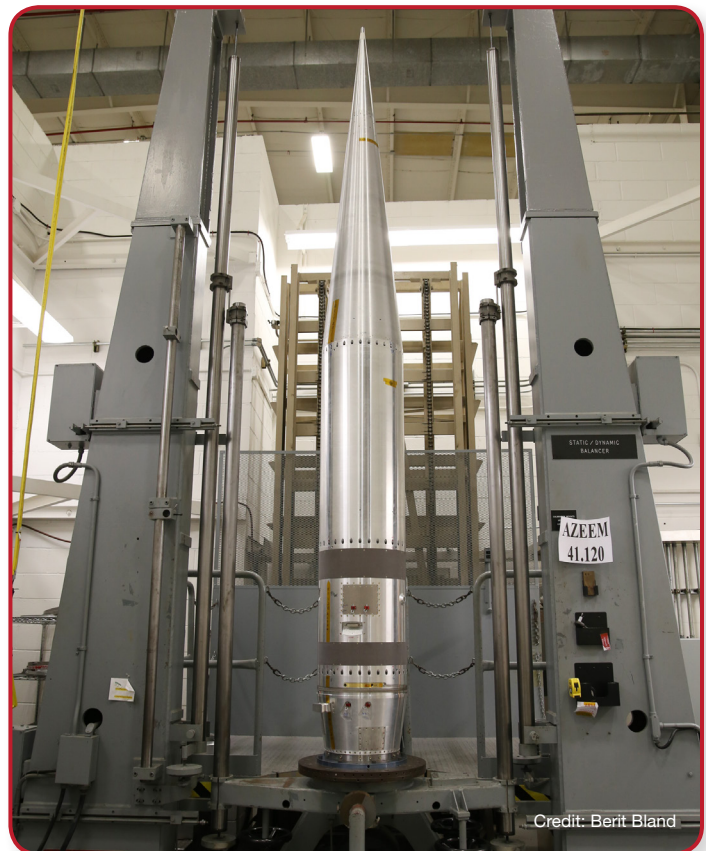
One of the three Super Soaker payloads undergoes spin/balance testing in the Sounding Rocket Payload Processing Facility at NASA's Wallops Flight Facility.
