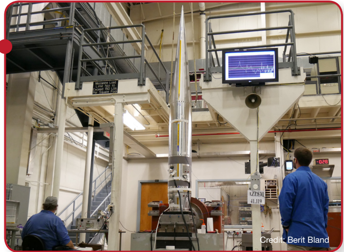
A Super Soaker payload is tested for its ability to operate while experiencing vibrations during flight.
