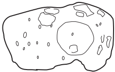
Asteroid
